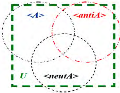
Fig. 5.3: Example of a particular neutrosophic diagram
