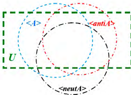
Fig. 5.2: Neutrosophic Diagram
