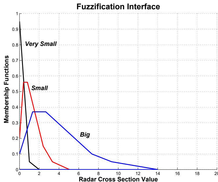
Figure 14.1: Fuzzification interface
