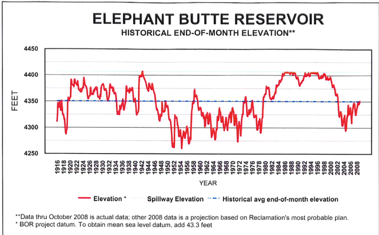
Figure 1. Historic end-of-month elevations for Elephant Butte Reservoir. (Elephant Butte Reservoir Five-year Operational Plan BA February 2009)
