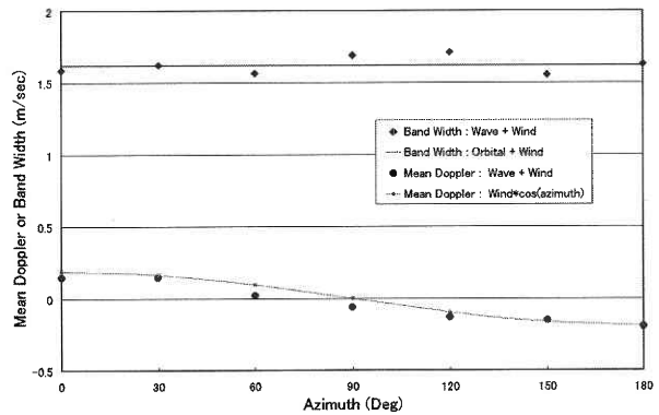
図9 Mean Doppler velocities and Doppler band widths
