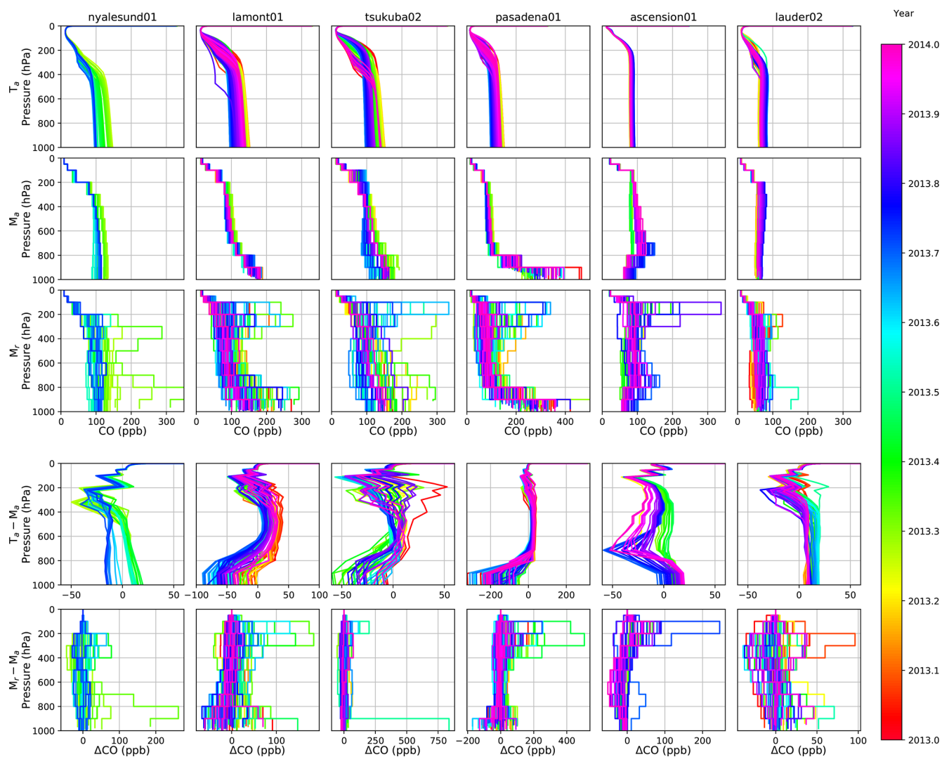
Figure D1. Profiles and profile differences between MOPITT and TCCON for six select sites and different days in 2013. For clarity, only one MOPITT profile within the coincidence criteria is selected per day. The rows are the TCCON a priori profiles ( T_a ), the MOPITT a priori profiles ( M_a ), the MOPITT retrieved profiles ( M_r ), the difference between TCCON and MOPITT a priori profiles, and the difference between MOPITT a priori and retrieved profiles.
