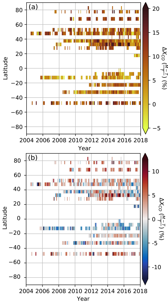
Figure 7. Rotated Hovmöller diagram of the mean percent differences between binned MOPITT and TCCON data using method II (Sect. S6.1). Latitude bins are 5° zonal bands, and temporal bins are monthly; (a) uses standard TCCON data, and (b) is without the TCCON scaling to aircraft (WMO scale – see Sect. S2).
