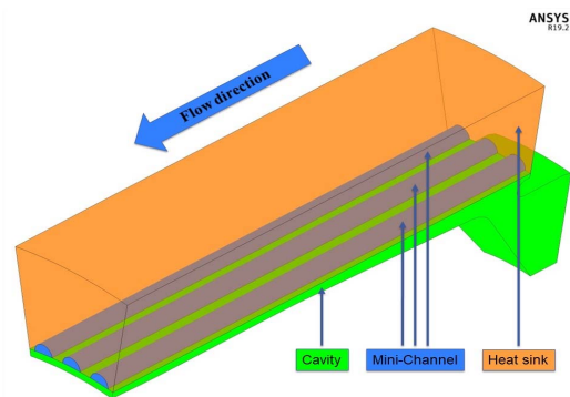
Fig. 1. Schematic view of the selected mini-channel cavity cooling
