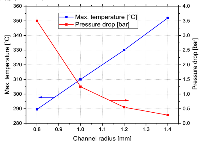
Fig. 2. Maximum temperature and pressure drop versus the channel radius.
