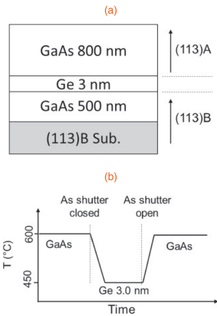
Fig. 2. (a) Epitaxial structure and (b) growth sequence for GaAs/Ge/GaAs heterostructure on (113)B GaAs.
