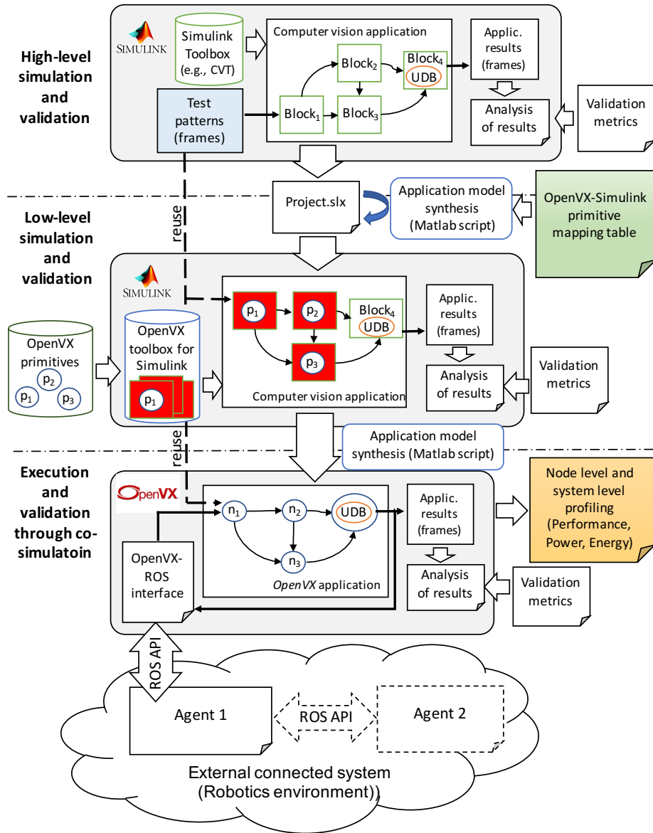
Fig. 3. Methodology overview
