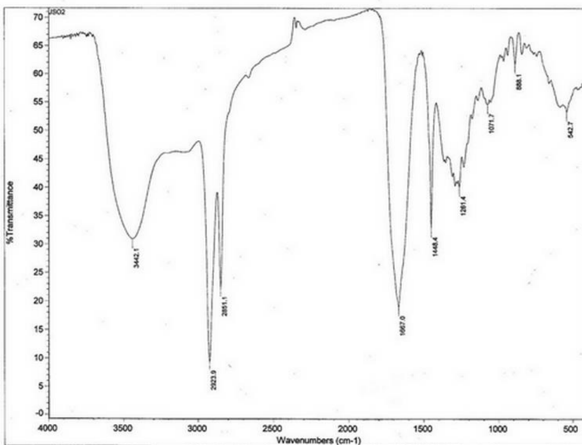
Figure S1. IR spectrum of [Pt(L)Br 2 ].
