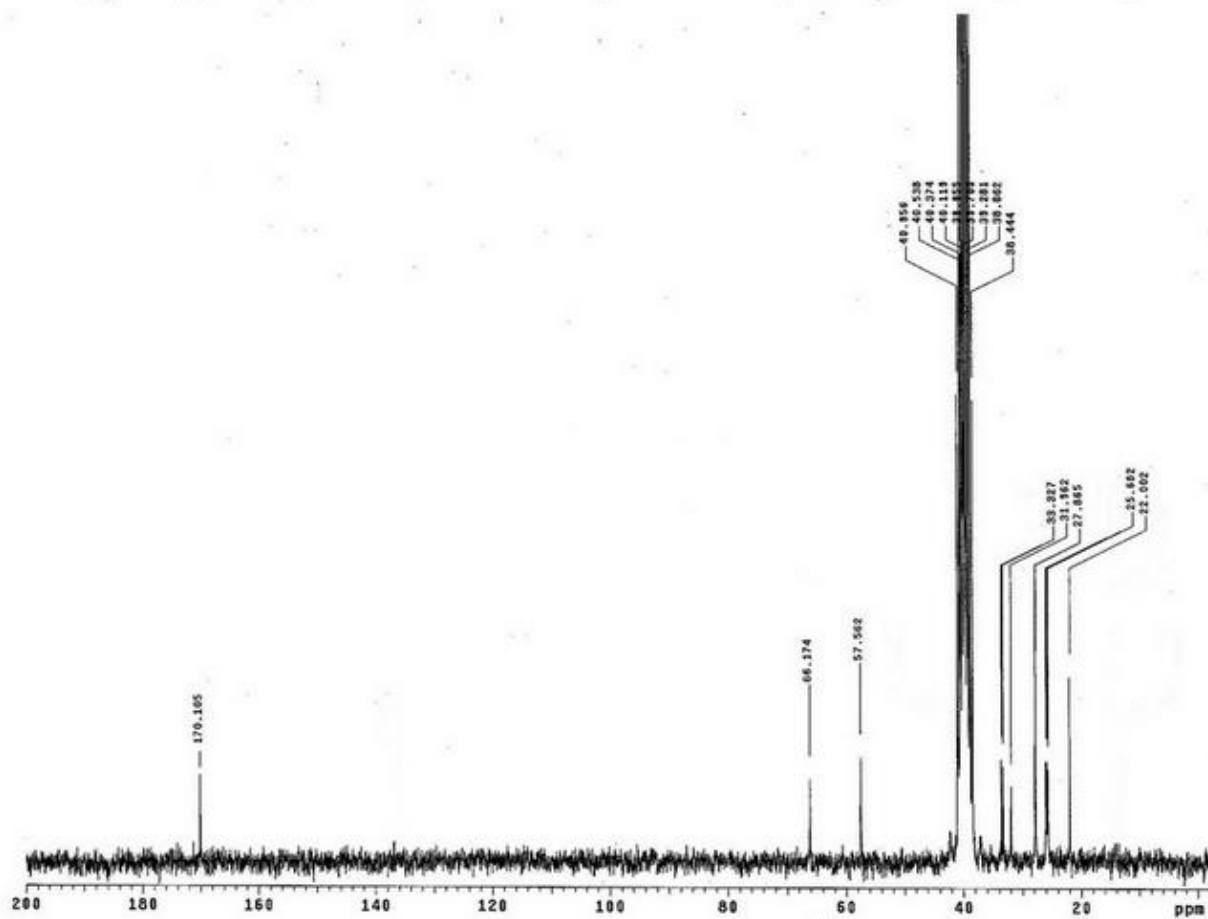
Figure S3. ^{13}\text{C} NMR spectrum of [\text{Pt}(\text{L})\text{Br}_2] .
