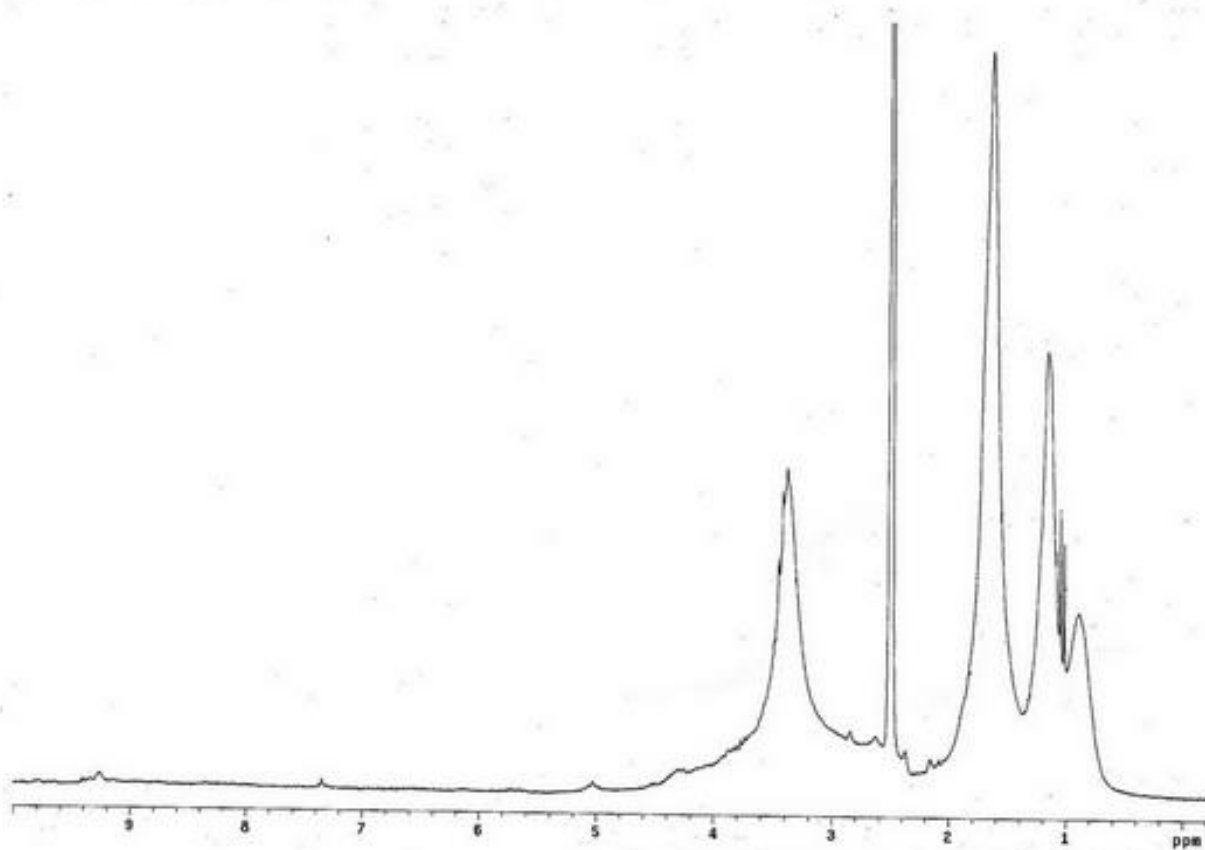
Figure S2. ^1\text{H} NMR spectrum of [\text{Pt}(\text{L})\text{Br}_2] .
