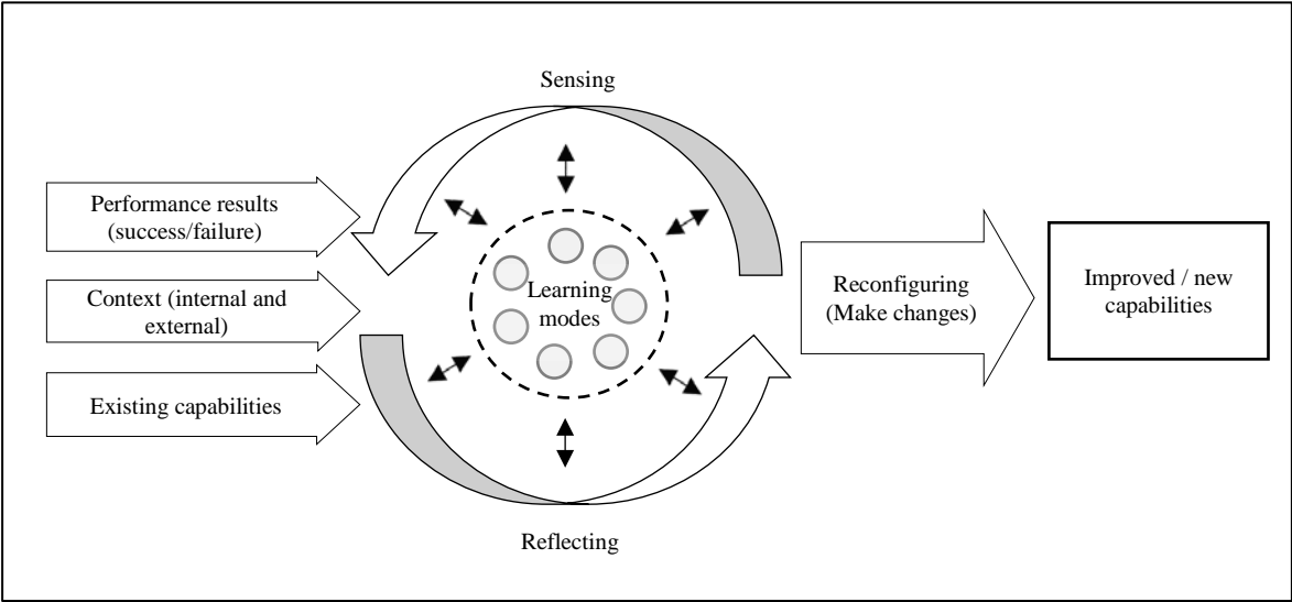
Figure 3- Learning Capability
