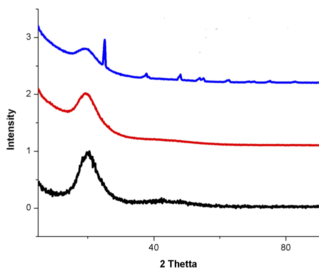
Figure 3 XRD images of a) PE (black line), b) PE/WG (red line) and c) PE/WG/TiO 2 (blue line). Sample with size of 1 cm * 1 cm was cut and recorded in Rigaku having CuK \alpha radiation in angle between 10° and 90°.
