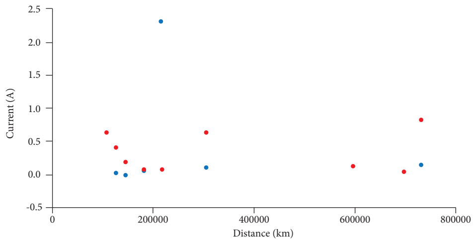
Figure 14. Solar array current of one array on square face (A) and three arrays on hexagonal face (B) of Shinen-2 micro deep-space probe, obtained from spacecraft telemetry.
