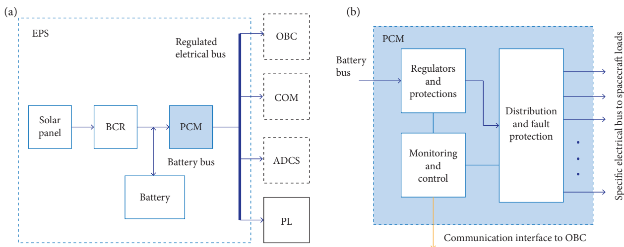
Figure 1. (a) Architecture of simple electrical power system on a small spacecraft and its interfaces with other subsystems. (b) Block diagram of a PCM indicating functional components.
