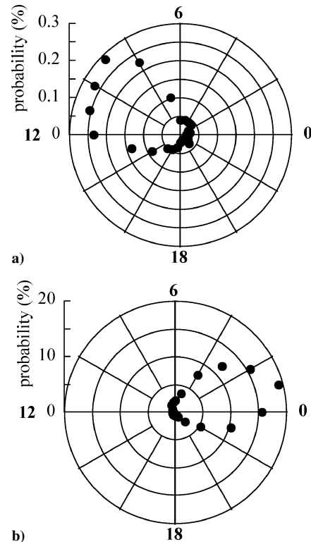
Fig. 9 Probability of occurrence for a) n_e > 10 \text{ cm}^{-3} and b) T_e > 3 keV observed on LANL satellites at each local time. The data during the eclipse are not included.
