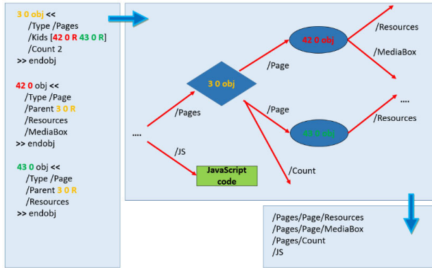
FIGURE 7. Example of the conversion of a PDF document to a set of structural paths.
