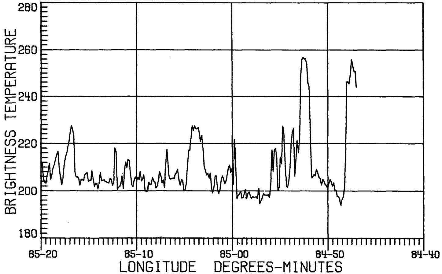
Figure 5-8. Radiometric brightness temperature of lake ice versus longitude for line 4.
