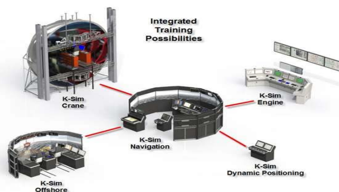
Figure 11 K-Sim Navigation and Integrated System
