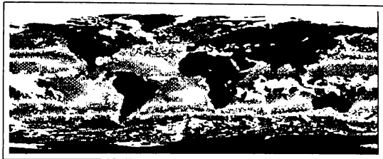
Figure 5. AVHRR satellite image. Monthly composition of the sea surface temperature from NOAA/NASA AVHRR Oceans pathfinders SST data set.
