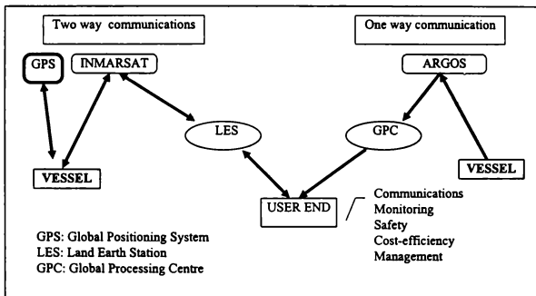
Figure 18. Monitoring system comparison (one and two way communications)
