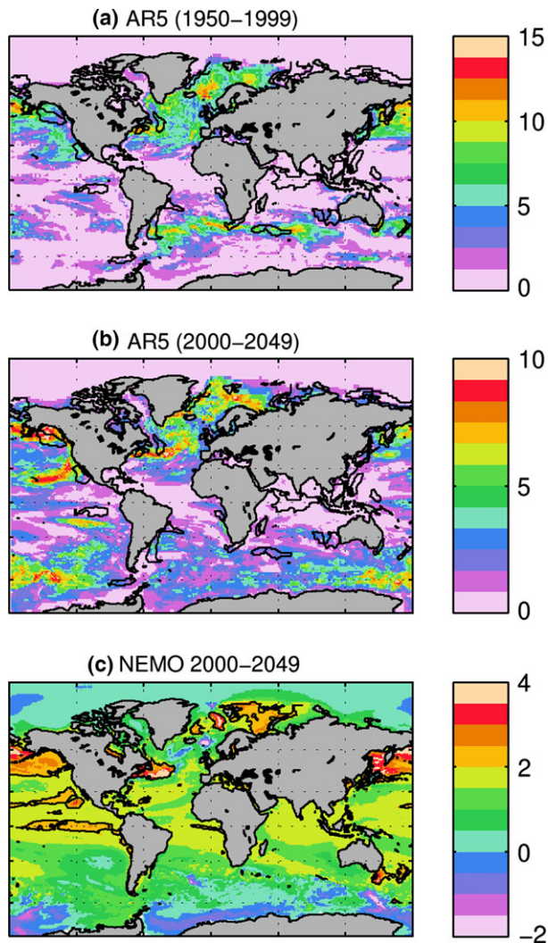
Fig. 1 (a) Overlap in occurrence of hotspots based on the historical (1950–1999) linear SST trend from 23 models used in CMIP5. The colour bar represents the number of models with a hotspot at the pixel location. Hotspots are identified as 10% of the fastest warming areas. (b) The same as (a) but for 2000–2049 period under RCP8.5 scenario; (c) SST linear trend in NEMO for 2000–2049 ( ^{\circ}\text{C} per 50 yr). Black contours on subplots a, b show hotspots identified in the same way by HP14 on the basis of historical observations. Black contours on subplot c show hotspots identified in the same way by HP14 on the basis of NEMO linear trend for 2000–2049.
