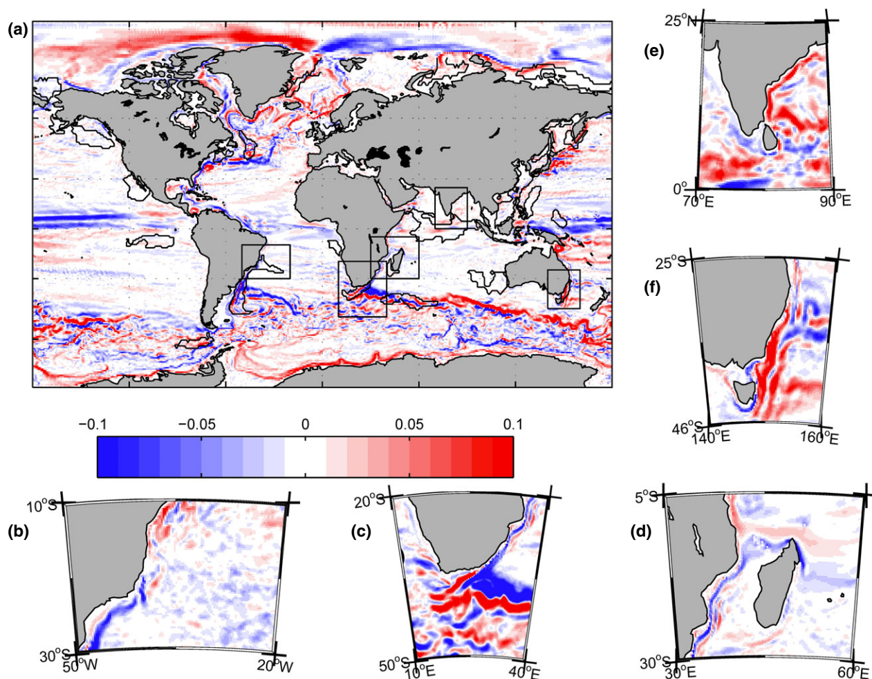
Fig. 2 Relative deviation of the decadal-averaged surface current speed of 2000–2009 from 2050 to 2060. (a) global distribution; magnified view for five regional hotspots: Brazilian (b) South African (c), Mozambique Channel (d), Indian (e) and East Australian (f).
