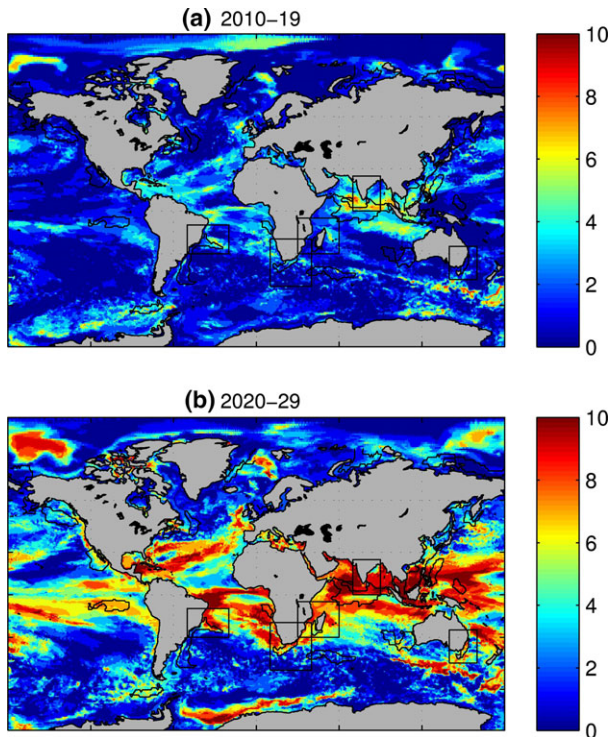
Fig. 4 Number of years in a decade 2010–2019 (a) and 2020–2029 (b) when annual SST falls outside of the range of its recent variability.
