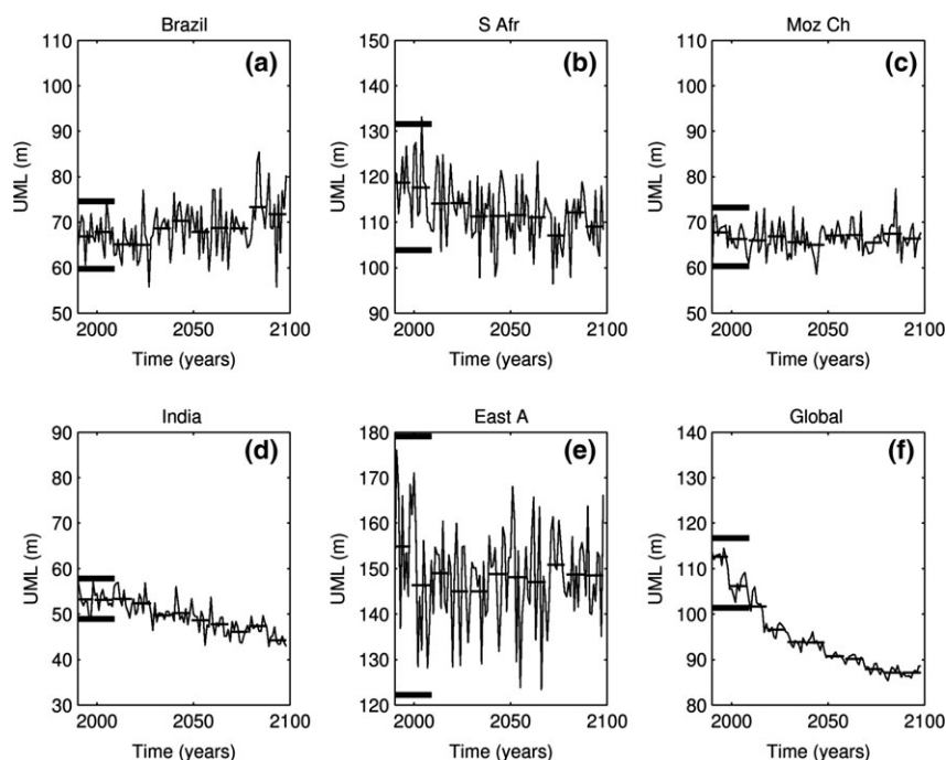
Fig. 5 Same as Fig. 3 for maximum UML depth (m).
