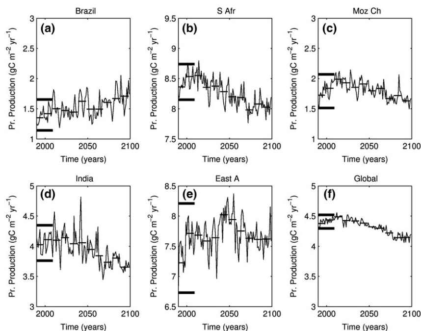
Fig. 6 Same as Fig. 3 for annual primary production ( \text{g C m}^{-2} \text{ yr}^{-1} ).
