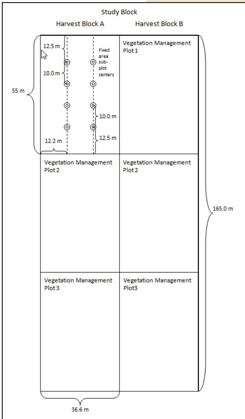
Figure 10. Layout and dimensions of study blocks, harvest treatment blocks, vegetation management treatment plots, and permanent fixed-area sub-plot centers.
