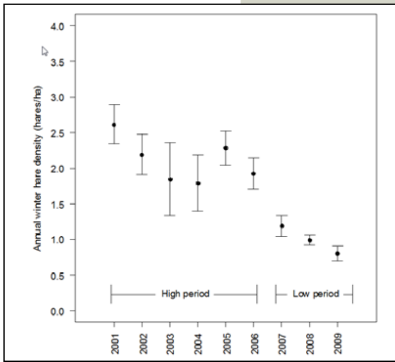
Figure 25. The mean and standard error (whiskers) of estimates for mean over-winter hare densities in 15 regenerating conifer stands in northern Maine, 2001-2009. Results of analyses indicate that hare populations fluctuated from a period of relatively high density (2001-2006; average 2.1 hares/ha) to relatively low density (2007-2009; average 1.0 hares/ha).
