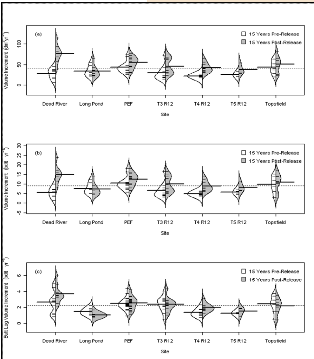
Figure 5. Beanplot of pre- and post- release volume increments by site, (a) for whole tree merchantable volume ( \text{dm}^3 \text{yr}^{-1} ), (b) Whole tree merchantable volume ( \text{bdf t yr}^{-1} ), and (c) butt log merchantable volume ( \text{bdf t yr}^{-1} ). Small horizontal lines represent individual observations, and large horizontal lines represent site means. Dashed line across entire figure represents grand mean.
