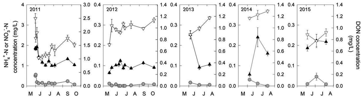
FIG. 15. Concentrations of \text{NH}_4^+ -N (black triangles), \text{NO}_3^- -N (gray circles), and DON (white inverted triangles) at the top of the bog water table. Values are means \pm SE ( n = 3 ). Arrows along the x-axes indicate N addition dates. Note the different y-axis scales for N concentrations for 2011 than for 2012–2015.
