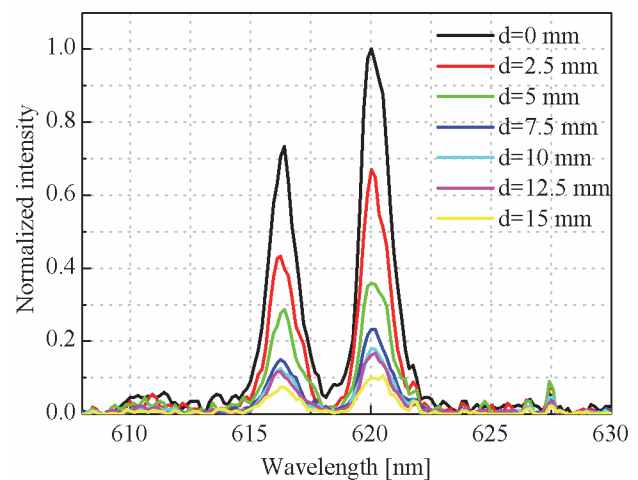
Fig. 10. Comparison of spectra on the output of the fiber-optic sensor with powder from mercury lamp in dependence on sensor distance from UV lamp 1.
