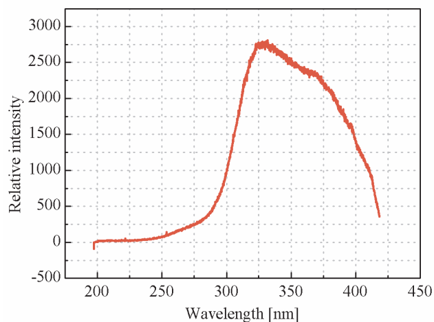
Fig. 6. UV spectrum of solar simulator.
