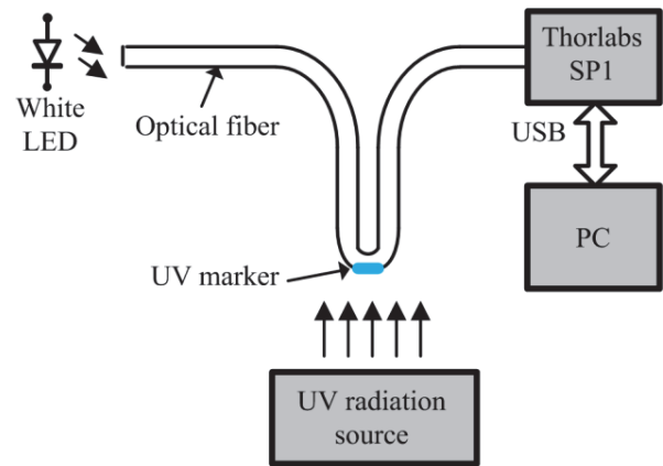
Fig. 1. The block diagram of experimental setup for fiber-optic UV radiation sensor based on U-shaped optical fiber.
