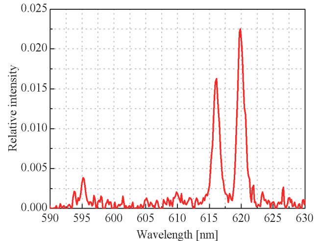
Fig. 9. Spectrum of fluorescent emission on the output of the fiber-optic sensor with powder from mercury lamp.
