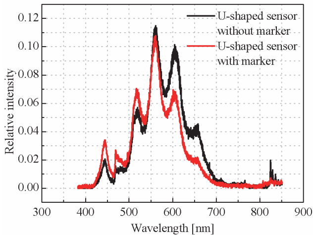
Fig. 7. Comparison of light spectra measured on the output of U-shaped sensor for cases with and without applied UV marker.
