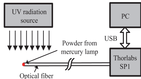
Fig. 3. The block diagram of experimental setup for end-type fiber-optic UV radiation sensor.
