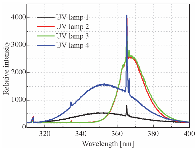
Fig. 8. Spectra of UV lamps used in experiments.
