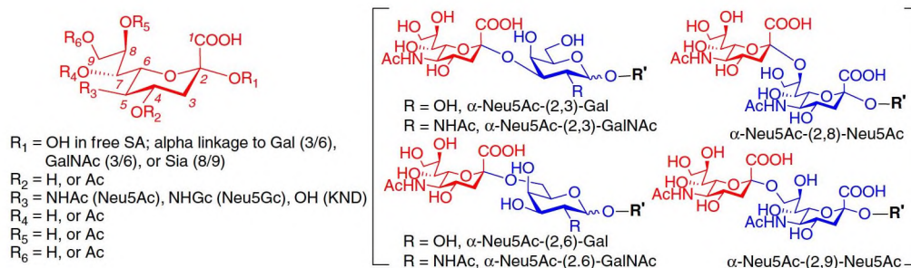
Fig. 1. Structures of sialic acids (SAs) and their natural linkages.
