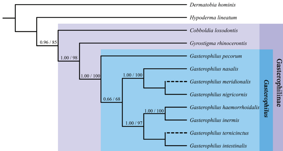
Fig. 2. Phylogeny of stomach bot flies inferred from mitogenomic data. Dashed branches indicate taxa placement based on morphological characters only. Numbers at the nodes are posterior probabilities (Bayesian trees)/bootstrap values (maximum likelihood trees) for molecular phylogeny construction. [Colour figure can be viewed at wileyonlinelibrary.com ].
