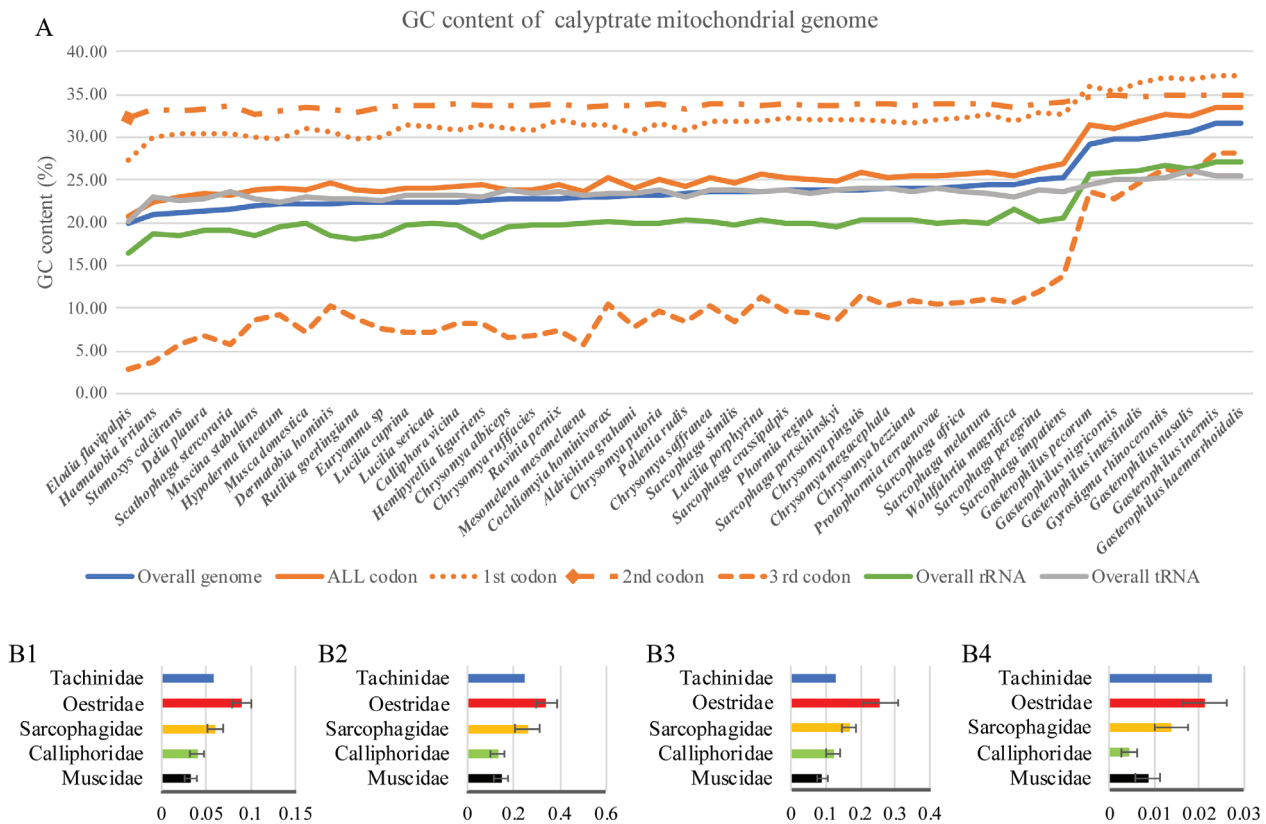
Fig. 1. Base composition and family-specific substitution rate of 13 mitochondrial protein-coding genes in calyprates. (A) Guanine and cytosine (GC) content of calyprate mitogenomes; (B1) mean evolutionary rates of each family estimated by dividing total amount of the Tamura–Nei substitution by divergence times; (B2) mean evolutionary rates of each family estimated by dividing total amount of substitution at fourfold degenerate sites by divergence times; (B3) mean evolutionary rates of each family estimated by dividing total amount of synonymous substitution by divergence times; (B4) mean evolutionary rates of each family estimated by dividing total amount of nonsynonymous substitution rates into divergence times. Error bars represent standard deviation from data of multiple species pairs. [Colour figure can be viewed at wileyonlinelibrary.com ].
