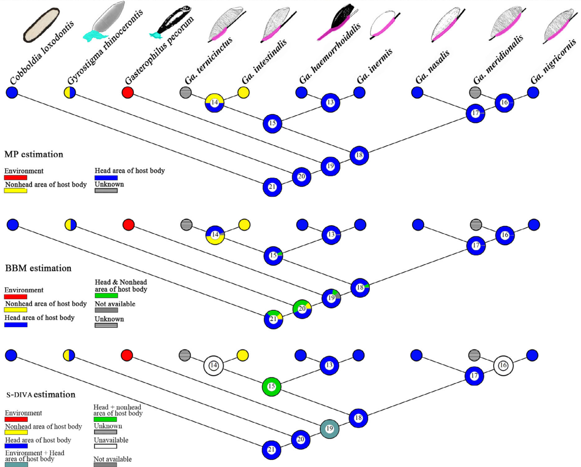
Fig. 4. Reconstructions of ancestral oviposition sites of stomach bot flies. Cladograms from top to bottom are reconstruction using maximum parsimony (MP), Bayesian binary Markov chain Monte Carlo (BBM) and STATISTICAL DISPERSAL-VICARIANCE ANALYSIS (s-DIVA), respectively. Possibility (MP) or probability (BBM and s-DIVA) for each node is shown as a colour proportion on the node. Eggs above cladograms are Cobboldia elephantis [this is the only egg of Cobboldia recorded in the literature (Patton, 1922)], Gyrostigma rhinocerontis , Gasterophilus pecorum , Gasterophilus termicinctus , Gasterophilus intestinalis , Gasterophilus haemorrhoidalis , Gasterophilus inermis , Gasterophilus nasalis , Gasterophilus meridionalis and Gasterophilus nigricornis , from left to right, with the structure of a type II attachment organ (AO) highlighted in Arctic blue, and that of a type I AO in pink. Known oviposition sites of each species are illustrated in the top picture using different colours. [Colour figure can be viewed at wileyonlinelibrary.com ].
