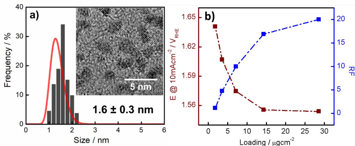
Figure 1. (a) Particle size distribution of the Ir NP determined from the HR-TEM micrographs and SAXS data. The insert displays a HR-TEM micrograph of the as synthesized Ir NP. (b) potential at a constant current density of 10 \text{ mA cm}^{-2} as a function of the theoretical Ir loading (- -■- -) and the RF established from the CO stripping data (- -■- -).
