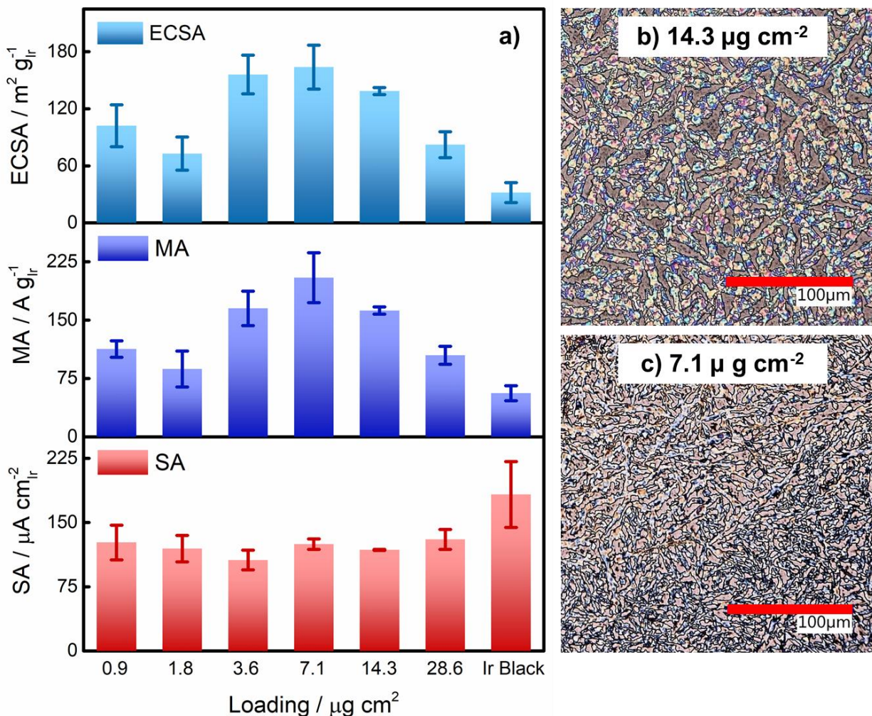
Figure 4. a) ECSA , Mass activity ( MA ) and specific activity ( SA ) as a function of Ir loading on the electrode. ECSA was determined by CO stripping . Loading for commercial Ir black is 7.1 \mu\text{g cm}^{-2} . All experiments were performed at room temperature. MA and SA were measured at 1.5 V_{\text{RHE}} during the positive going scan. b) and c) images taken with an optical microscope show NP deposited on the glassy carbon disks. The brown regions belong to the glassy carbon whereas the colorful network is produced by the NP.
