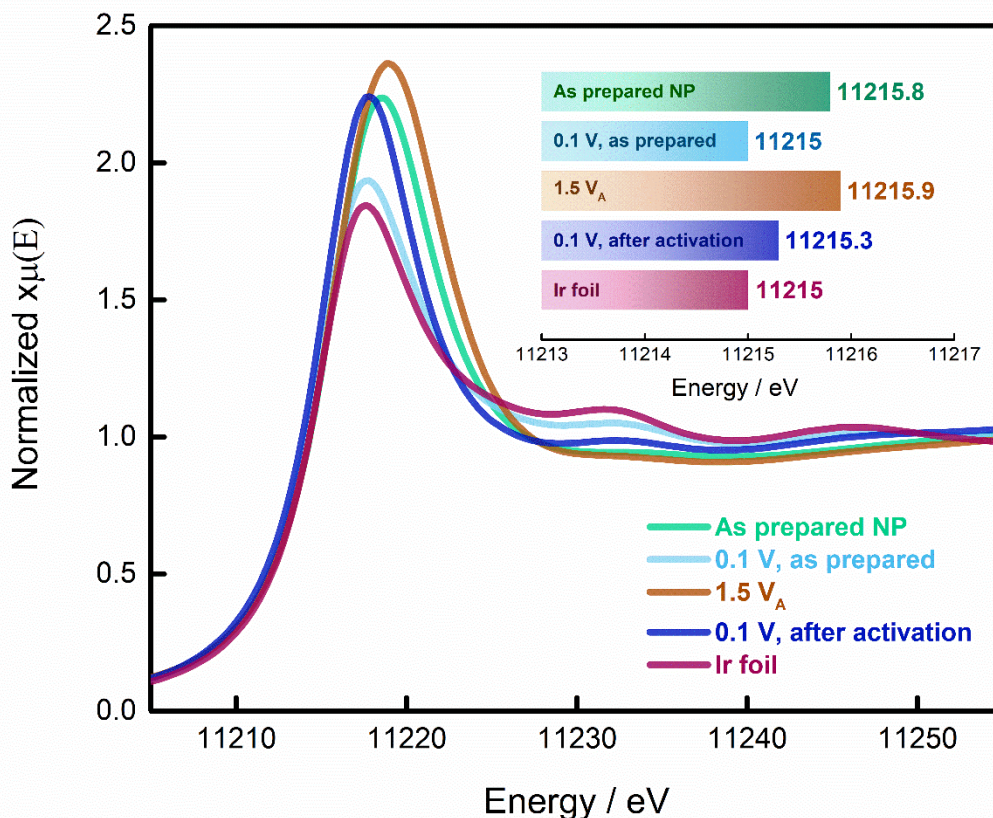
Figure 3. Normalized Ir L_3 -edge XANES spectra for the Ir NP recorded at different potentials under steady state conditions. V_A stands for “anodic”. The insert displays the energy at the maximum of the first derivative of the XANES spectra for the different samples. The density of the datapoints in the plots is 5 points/eV.
