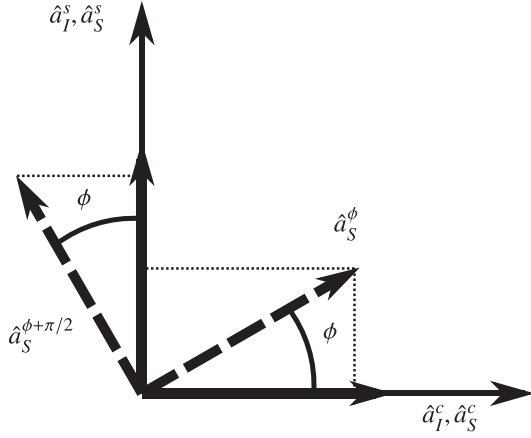
FIG. 2. Geometrical representation of the virtual rigidity effect. The backaction and imprecision noise quadratures for I and S are depicted with respect to the quadrature bases (\hat{a}_{I,S}^s, \hat{a}_{I,S}^c) , respectively. Homodyne measurement quadratures are chosen to be \hat{b}_I^s and \hat{b}_S^s (i.e., \zeta_I = \zeta_S = \pi/2 ) so that the corresponding imprecision noise quadratures (vertical bold arrow) coincide with the vertical axes, \hat{a}_I^s and \hat{a}_S^s . For I , we make the “standard” choice of probe phase \phi_I = 0 such that the orthogonal quadrature \hat{a}_I^c acts as backaction. However, for S , a probe phase \phi = \phi_S relative to \hat{a}_S^c is introduced.
