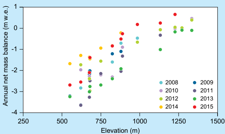
Figure 2. Surface mass balance observations from the GEM GlacioBasis ablation stakes network on A.P. Olsen ice cap, NE Greenland. Data for 2016 becomes available after the 2017 field campaign.
