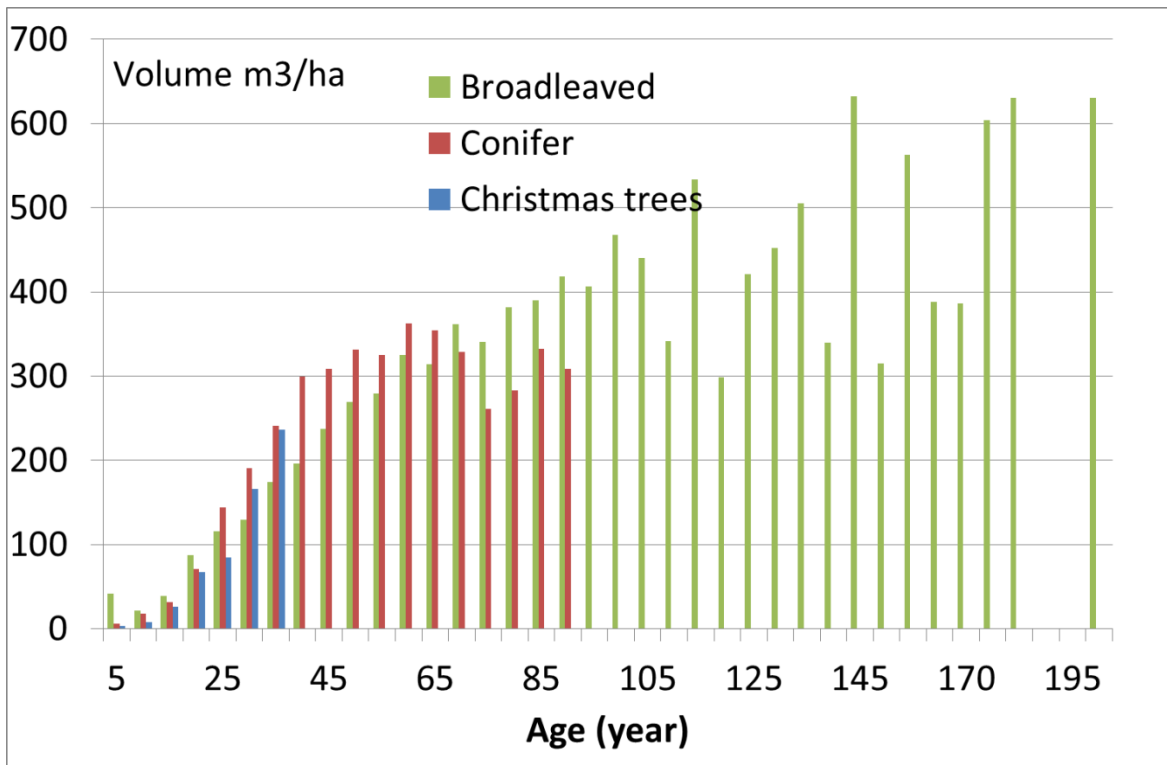
Figure 19 Growing stock (above ground biomass m^3 ha^{-1} ) by age class distribution by 2010, for broadleaved, conifers and Christmas trees.
