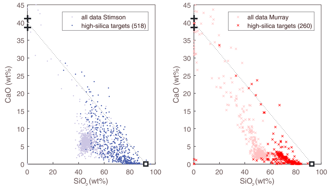
Figure 8. Silica content as a function of calcium oxide content for targets of the Stimson and Murray formations. Data from targets, which include one or several points with more than 65 wt% \text{SiO}_2 and less than 3 wt% CaO, are represented for the Stimson (bold blue dots) and Murray (bold red crosses). The total number of points from these targets is shown in the legend: 518 for Stimson and 260 for Murray. The remaining target data are shown in lighter color (Stimson: pale blue dots, Murray: pale red crosses). Note that this data set deliberately includes all points, whereas data shown on Figure 5 were classified to remove points with a contribution from Ca-sulfates (Frydenvang et al., 2017). Reference compositions of opal with 6 wt% water (black square), as well as anhydrite -\text{CaSO}_4- and bassanite -\text{CaSO}_4 \times 0.5\text{H}_2\text{O}- (black crosses), are shown along with mixing trend (dotted line).
