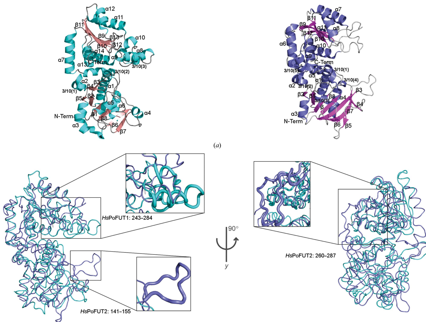
Figure 2 (a) Cartoon representations of the human PoFUT1 (PDB entry 5ux6; McMillan et al. , 2017) and PoFUT2 (PDB entry 4ap5; Chen et al. , 2012) structures. Secondary structures are shown for HsPoFUT1 with helices in cyan and β-sheets in salmon; for HsPoFUT2 helices are shown in slate blue and β-sheets in magenta. (b) Superimposed structures of HsPoFUT1 (cyan) and HsPoFUT2 (slate blue). Main secondary-structure differences are highlighted in boxes.
