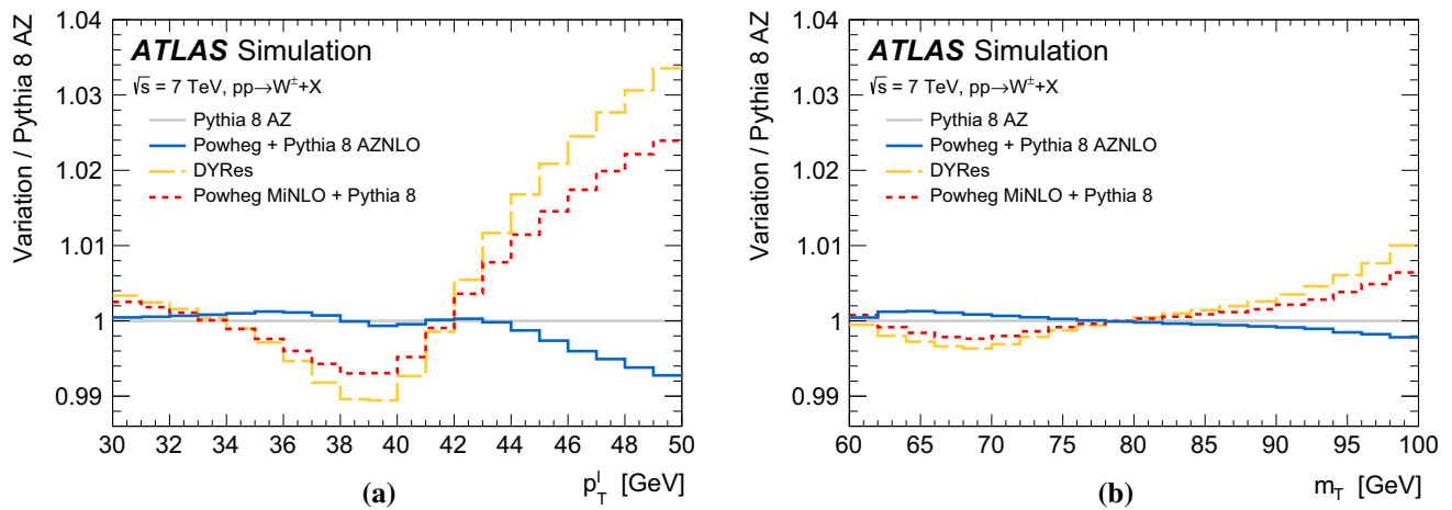
Fig. 2 Ratios of the reconstruction-level a p_T^\ell and b m_T normalized distributions obtained using POWHEG+PYTHIA 8 AZNLO, DYRes and POWHEG MINLO+PYTHIA 8 to the baseline normalized distributions obtained using PYTHIA 8 AZ
