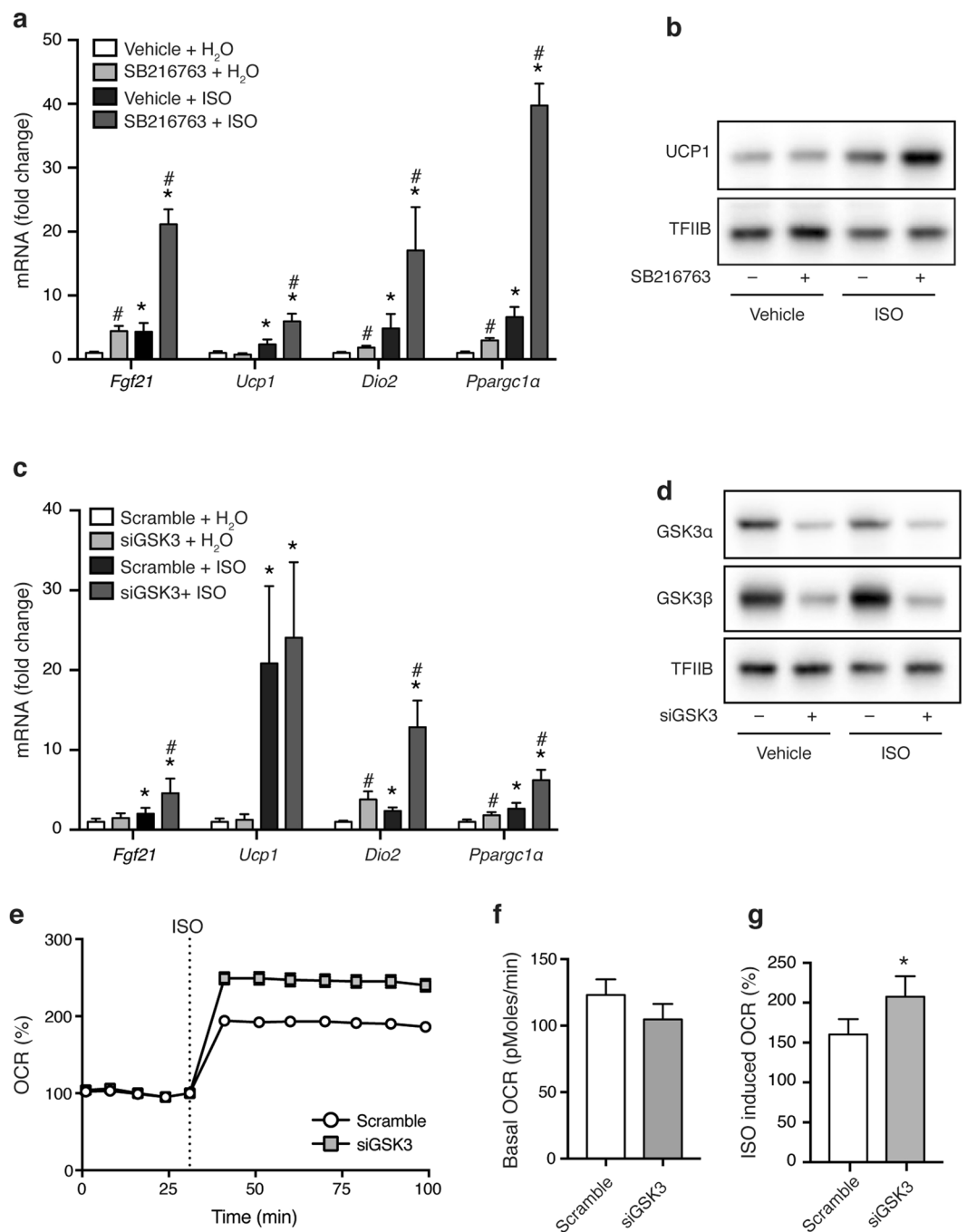
Figure 3. GSK3 restricts the thermogenic program in brown adipocytes. (a) Expression of thermogenic genes ( Fgf21 , Ucp1 , Dio2 and Pparg1a ) in primary brown adipocytes pre-treated with 10 \mu M SB216763 for 1 h before being stimulated with 0.1 \mu M ISO for an additional 6 h. (b) Immunoblot analysis of UCP1 in primary brown adipocytes pre-treated with 10 \mu M SB216763 for 1 h before being stimulated with 0.1 \mu M ISO for an additional 24 h. TFIIIB serves as loading control. (c) Expression of thermogenic genes ( Fgf21 , Ucp1 , Dio2 and Pparg1a ) in siRNA-transfected primary brown adipocytes stimulated with 0.1 \mu M ISO for 6 h. (d) Immunoblot analysis of GSK3 \alpha and GSK3 \beta in siRNA-transfected primary brown adipocytes stimulated with 0.1 \mu M ISO for 24 h. TFIIIB serves as loading control. (e) Representative normalized Seahorse run of oxygen consumption rates (OCR) in siRNA-transfected primary brown adipocytes. Quantification of basal (f) and ISO (1 \mu M)-induced (g) OCR. RT-qPCR data are presented as mean of means ( \pm SEM) ( n = 4 ). Statistical significance was determined by two-way ANOVA with repeated measures and Tukey's post hoc test for multiple comparisons. * p < 0.05 versus H 2 O. # p < 0.05 versus vehicle/scramble. Seahorse data are presented as mean ( \pm SEM) of one representative experiment (e) or 3 independent experiments (f,g) and significance was determined by paired t-test (* p < 0.05 ). For panels b and d, full-length blots/gels are presented in Supplementary Fig. 2.
