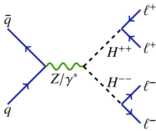
Fig. 1 Feynman diagram of the pair production process pp \rightarrow H^{++} H^{--} . The analysis studies only the electron and muon channels, where at least one of the lepton pairs is e^{\pm}e^{\pm} , e^{\pm}\mu^{\pm} , or \mu^{\pm}\mu^{\pm}
