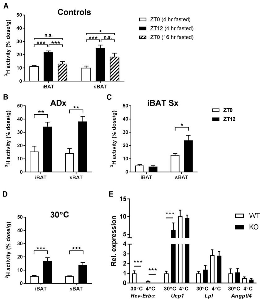
Figure 3. 24-Hr Rhythm of TG-Derived FA Uptake by BAT after Prolonged Fasting, Adrenalectomy, and Sympathetic Denervation at Thermoneutrality and in Rev-erb \alpha Null Mice (A–D) Wild-type mice were subjected to normal LE and injected with glycerol tri 3 H]oleate-labeled lipoprotein-like particles at lights on (ZT0) or lights off (ZT12). The uptake of [ 3 H]oleate was determined for interscapular BAT (iBAT) and subscapular brown adipose tissue (sBAT) after prolonged fasting (n = 8 per group; A), after adrenalectomy (n = 4–5 per group; B), after sympathetic denervation of iBAT (n = 8 per group; C), or after housing at thermoneutrality (n = 7 per group; D). (E) Gene expression in Rev-Erb \alpha null mice was compared to that of littermates housed at thermoneutrality or cold (n = 4–5 per group). Data are presented as means \pm SEM. *p < 0.05; **p < 0.01; ***p < 0.001, ANOVA with Tukey’s post hoc test in (A), independent-samples t test in (B)–(D), and two-way ANOVA with Tukey’s post hoc test in (E). n.s., not significant. See also Figure S4.
