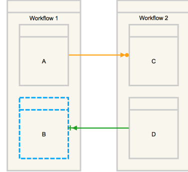
Figure 2: Inter-workflow relations
