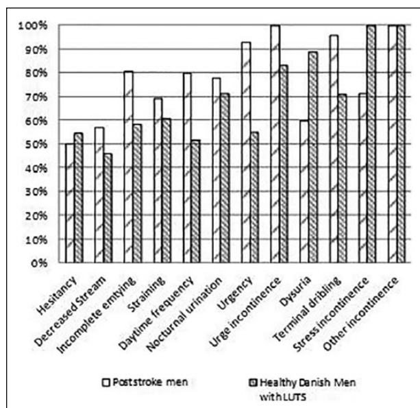
Figure 2. Prevalence of both of lower urinary tract symptoms (LUTS) in poststroke men compared with healthy men with LUTS.
