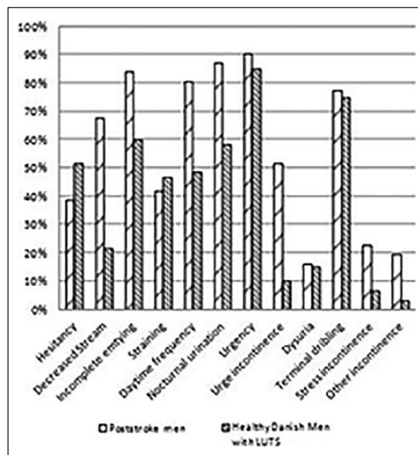
Figure 1. Prevalence of lower urinary tract symptoms (LUTS) in poststroke men compared with healthy men with LUTS.
