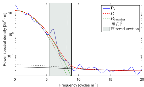
Fig. 6. The interference of the annual spectral signal is seen in the PSD of the \delta\text{D} GRIP mid Holocene section. The regular fit is represented by the solid lines and the dashed lines represent the case where the weight function w(f) has filtered out this artifactual bias.
