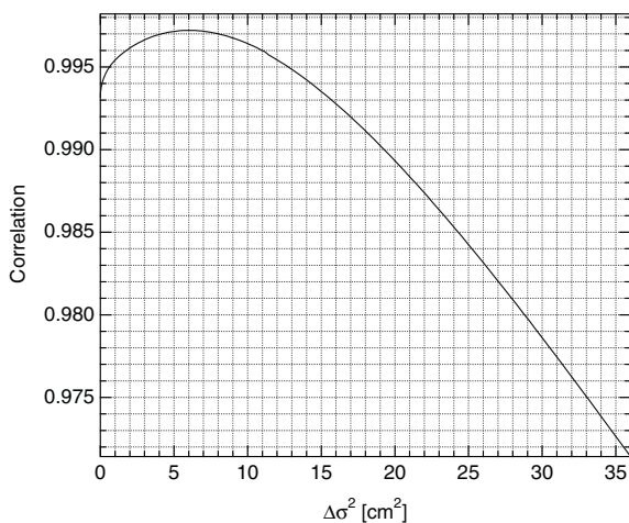
Fig. 9. Correlation coefficient ( r_{\delta^{18}O/\delta D} ) between the \delta^{18}O and the forward-diffused \delta D series as a function of the estimated ^{18}\Delta\sigma^2 . The synthetic data represent a case A climate.
