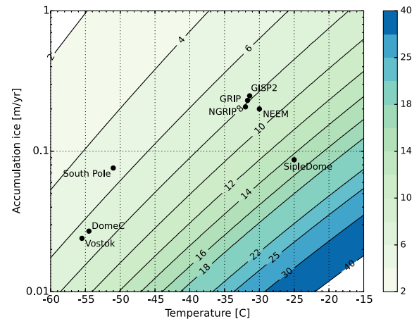
Fig. 2. Modeled firn diffusion lengths [cm] for \delta^{18}\text{O} as a function of temperature and accumulation rate (with \rho_{co} = 804 \text{ kg m}^{-3} and \rho_0 = 330 \text{ kg m}^{-3} ) from Gkinis et al. (2014). The contours indicate lines of constant diffusion length and the colorbar represents the diffusion length in cm. Here the combined impact of temperature and accumulation rate on the diffusion length is evident; while warm temperatures induce high diffusion lengths, a high accumulation rate reduces the diffusion length estimate. The firn diffusion lengths corresponding to a few ice core sites are plotted as a reference. (For interpretation of the references to color in this figure legend, the reader is referred to the web version of this article.)
