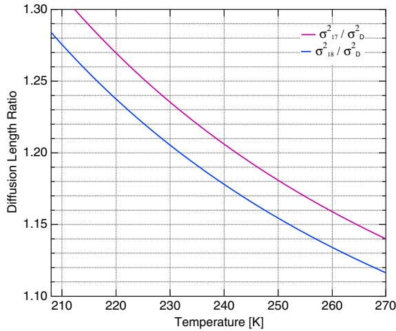
Fig. 10. The diffusion length ratios \sigma_{18}^2/\sigma_D^2 and \sigma_{17}^2/\sigma_D^2 with respect to temperature. The \sigma_{18}^2/\sigma_{17}^2 is almost constant at 0.975 and omitted here due to its very low temperature sensitivity.
