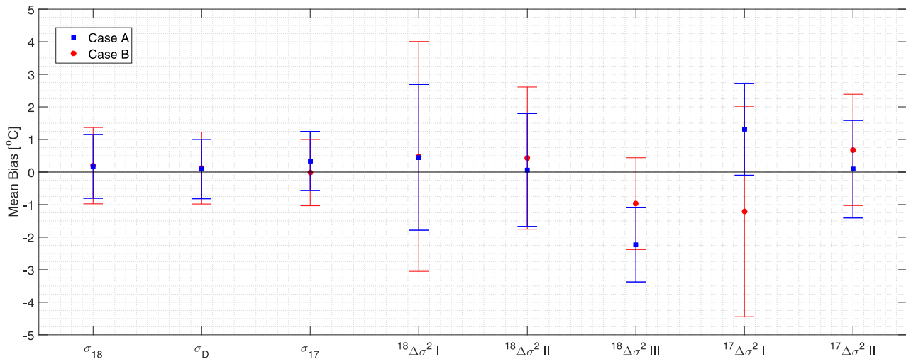
Fig. 11. Mean biases for the single and differential diffusion techniques. The error bars represent 1 std of the estimated temperatures.
