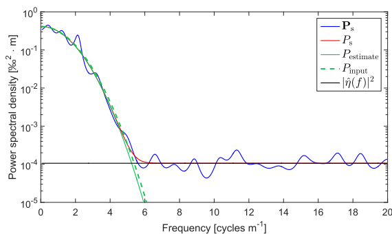
Fig. 5. PSD of a synthetic \delta^{18}\text{O} time series plotted with respect to frequency (blue curve). The red curve represents the complete model fit (Eq. (11)). The green dashed curve represents the input diffusion length and the solid green curve represents the estimated diffusion length of the signal (uncorrected for sampling diffusion). The black curve represents the noise part of the fit. (For interpretation of the references to color in this figure legend, the reader is referred to the web version of this article.)
