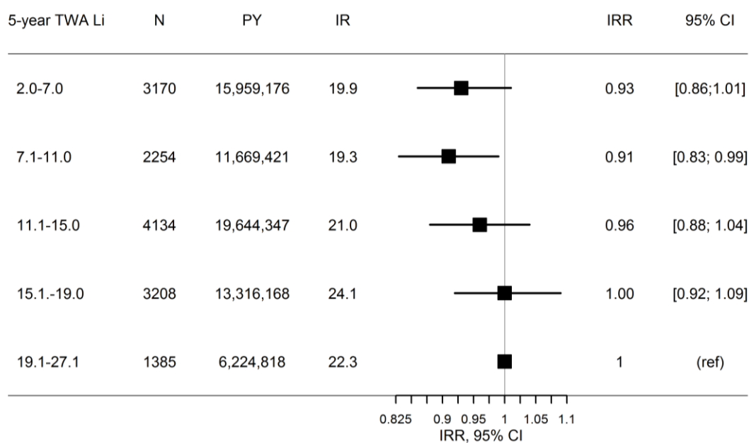
Figure 4. Incidence rate ratio (IRR) for suicide with increasing five-year time-weighted average (TWA) lithium exposure level (Li in \mu\text{g}/\text{L} ) in drinking water using a Poisson regression model with the random effect modelled using a conditional autoregressive model (CAR) adjusted for differences in gender, age, employment, civil status, and calendar year. N: number of suicides; PY: person-years at risk; IR: crude incidence rate; IRR: adjusted incidence rate ratio; 95% CI: 95% credible interval; ref: reference group. The spatial regression analysis was performed in R Version 3.2.2 using the INLA package [40].
