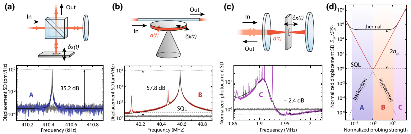
Fig. 1 Probing mechanical motion \delta x(t) by laser interferometry. a Simple two-path interferometer, involving reflection off the mechanical device ( top ). The thermal motion ( blue trace ) of a high- Q membrane is readily resolved above the measurement imprecision background ( gray ). b Cavity-enhanced measurement, here of a radial-breathing mode of an optical whispering-gallery-mode resonator ( top ). Thermal motion ( red trace ) is far above the imprecision background ( gray ), which is itself below the resonant standard quantum limit (SQL) for this mechanical mode (from [10]). c Cavity-based
