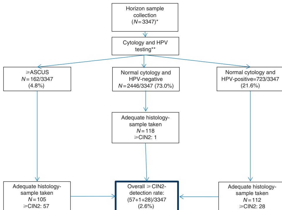
Figure 2. Flowchart of the Horizon study design, follow-up triage, and \geq CIN2 detection. *Of the 3347 screened women, 16 (0.48%) were inadequate for cytology reading. One of the women had a histology sample registered with normal findings. This contributed to a total of 336 biopsies taken. **Women were followed-up according to routine practice based on the cytology result only. An active follow-up was performed on women with cytology normal HPV-positive findings according to the study protocol that was repeat testing after 18 months. Women with normal cytology and negative HPV test results were referred back to the routine screening programme; some of these had a histology sample taken despite the recommendations. Women who were cytology negative and HPV positive were invited for repeated testing after 18 months. All HPV test results reported here took into account the testing results on any of the four assays. CIN = cervical intraepithelial neoplasia.
