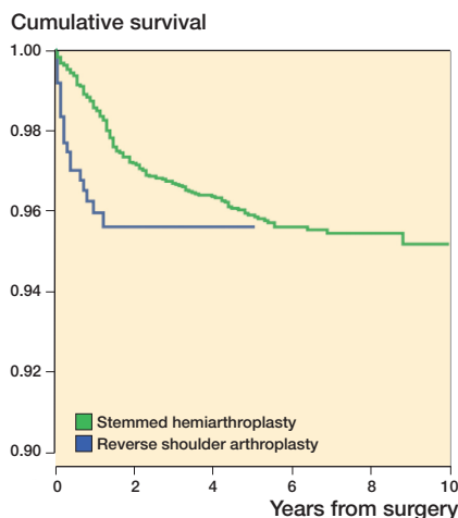
Figure 2. Cumulative survival over the years.
