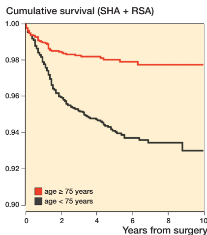
Figure 4. Cumulative survival of both SHA and RSA over the years in 2 age groups.
