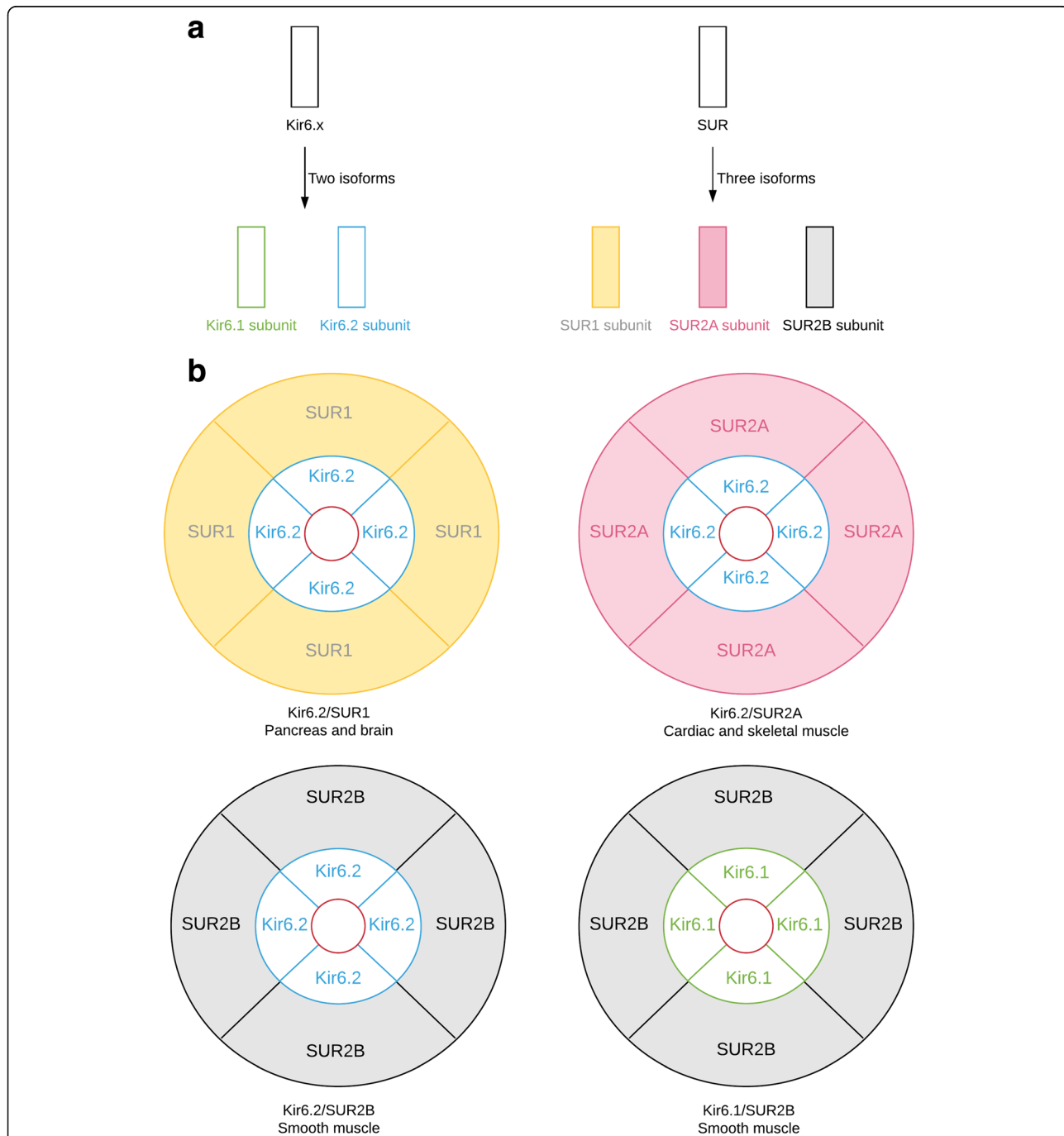
Fig. 1 Molecular structure and isoforms. a Two major Kir6.x isoforms (Kir6.1 and Kir 6.2) and three major SUR isoforms (SUR1, SUR2A and SUR 2B) have been identified. b Kir.x subunits combine tissue-specifically with different SUR subunits to form various native K_{ATP} channels. Pancreatic, cardiac and smooth muscle K_{ATP} channels are made up of Kir6.2/SUR1, Kir6.2/SUR2A and Kir6.1 (or Kir6.2)/SUR2B, respectively [2]. Kir, inwardly rectifying K^+ channels; SUR, sulfonylurea receptor
