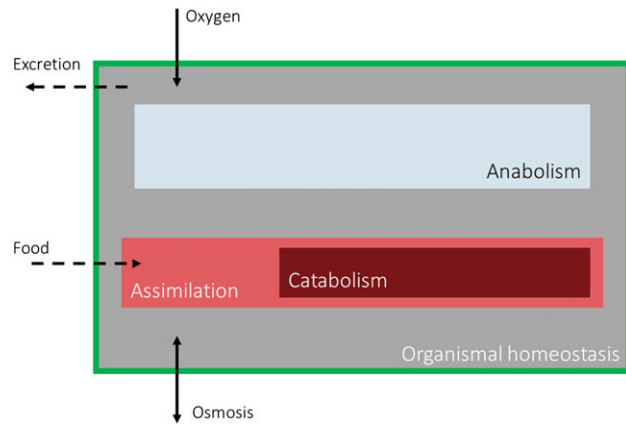
Figure 2: Energy budget of a resting fish. Organismal homeostasis, grey, is here depicted as 60% of the total expenditure (150 cm 2 ), the primary constituents being convective ‘oxygen transport’ (branchial + cardiac) and ‘osmoregulation’. Behaviour and similar activities are not included here, as the fish is at rest. Assimilation of food to utilizable energy is represented in this situation at a level of ≈18.3 % of the total budget (27.5 cm 2 ), of which catabolism uses 45% (representative of Alanine) (Applebaum & Rønnestad (2004), Rønnestad et al. (2001)). Lastly anabolism, i.e. growth, consists of ≈22% (32.5 cm 2 ). The given situation leaves room for growth in the sense of Von Bertalanffy (1934) since anabolism is larger than catabolism (assimilation). The green line represents any surface of the organism, where uptake of oxygen and exchange of water and ions occur.
