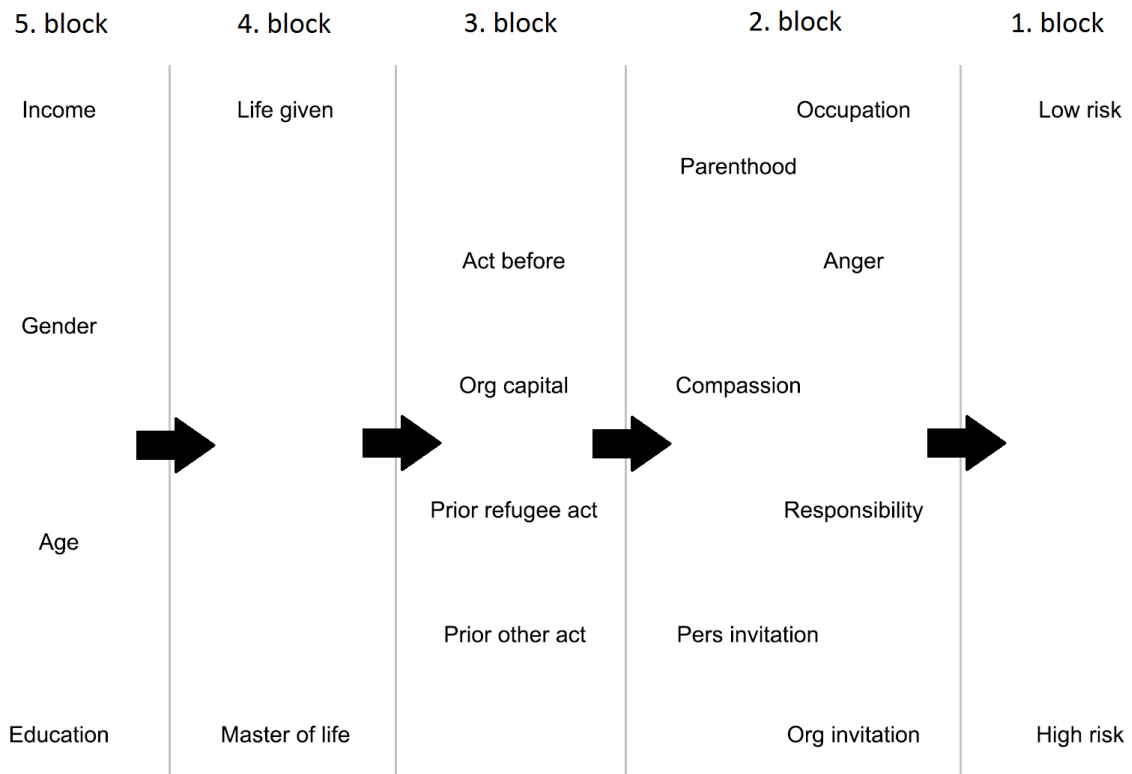
Figure 7.2. Recursive block model
