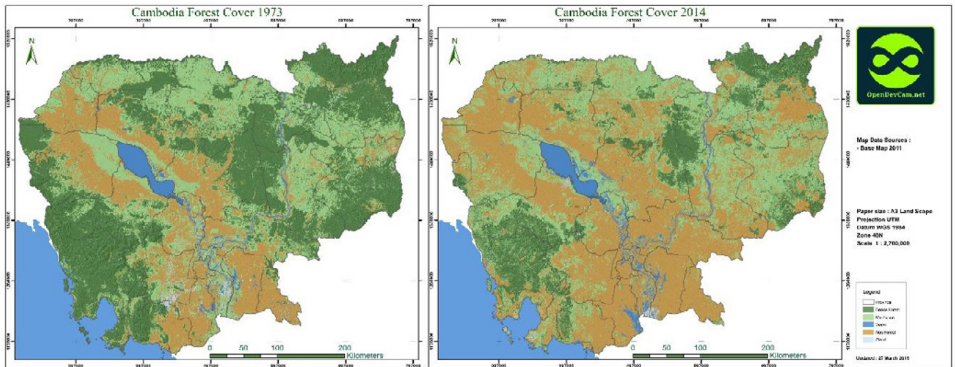
Figure 1.1: Forest loss in Cambodia. Generated from maps provided by Open Development Cambodia ( https://opendevlopmentcambodia.net/layers ).
