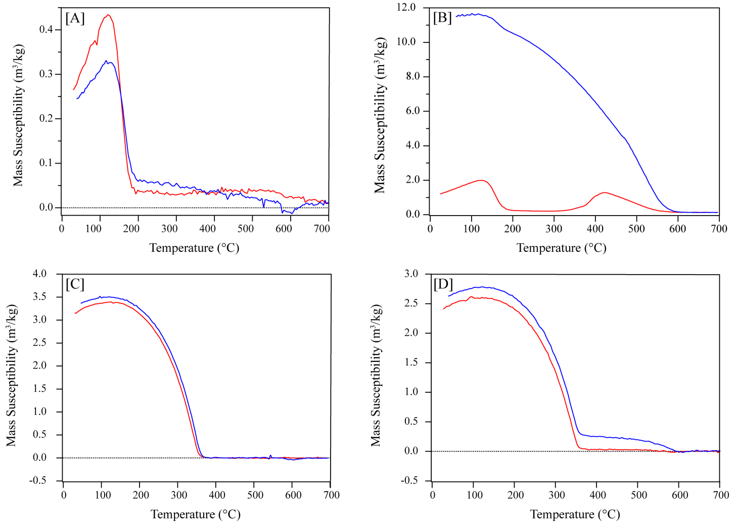
Fig 5. Thermomagnetic curves which illustrate the Curie temperature for: [A] CNT-Wako, [B] MCNT-Wako, [C] CNT-Alpha, and [D] MCNT-Alpha. Red/blue shows the heating/cooling curves, respectively.
