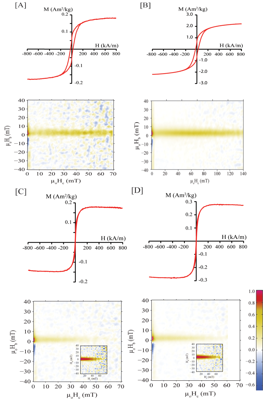
Fig 4. Magnetization curves up to 796 kA/m at 293 K and FORC diagrams for: [A] CNT-Wako, [B] MCNT-Wako, [C] CNT-Alpha, and [D] MCNT-Alpha. Inset in the FORC diagrams show the contribution of the higher coercivity for the Alpha samples.
