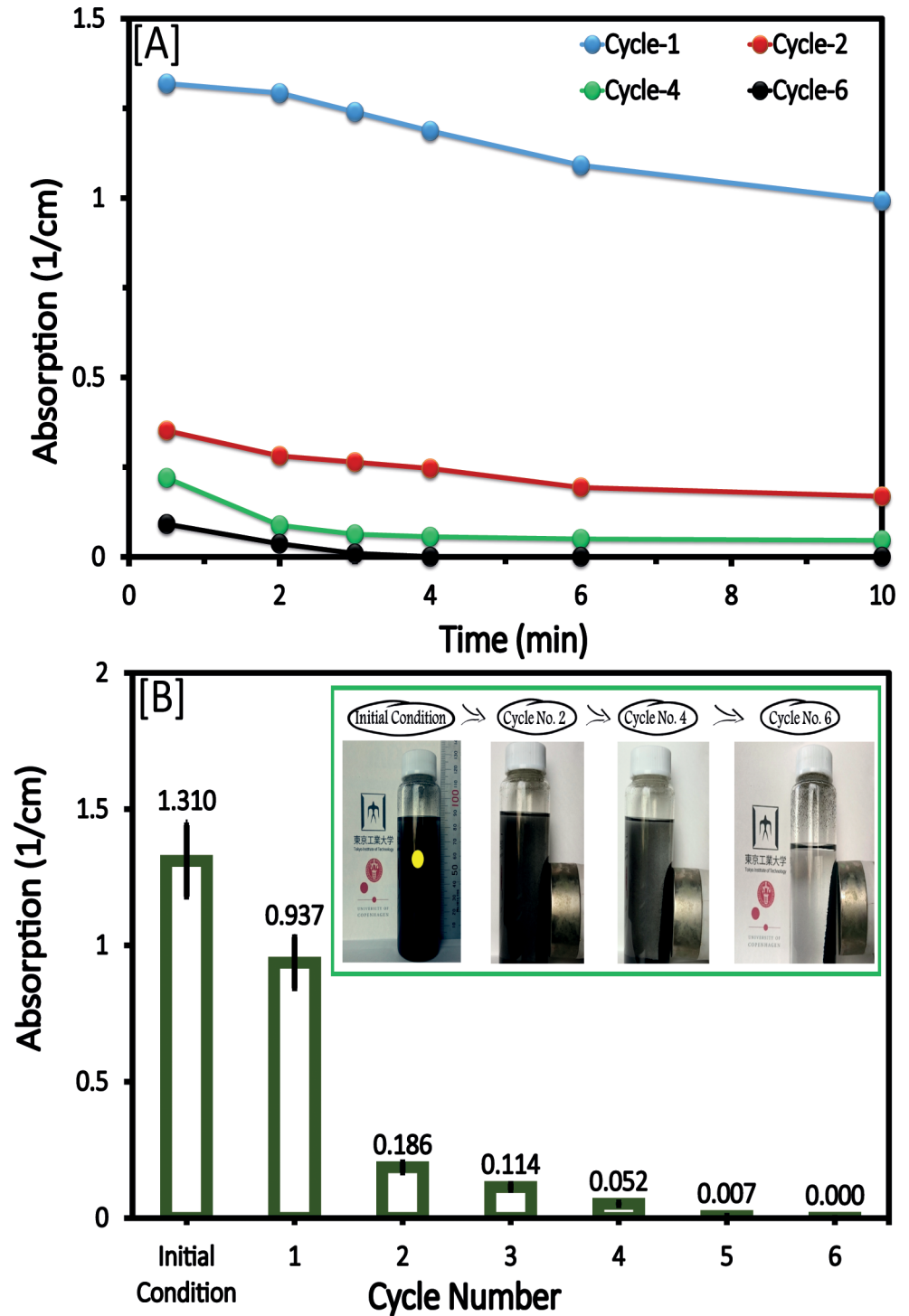
Fig 1. Absorbance at 800 nm of the supernatant (center of the vial) during the magnetic separation cycle. Panel [A] illustrates the MCNT collection efficiency as a function of time, and panel [B] shows the final residual amounts of magnetic CNT in the supernatant 10 min after introducing a permanent magnet adjacent to the suspension. Vertical lines are standard error bars from 3 replicates. Inset: Pictures taken at the end of the upgrading cycle (10 min after introducing the suspension to a permanent magnet). The yellow dot indicates the sampling point.
