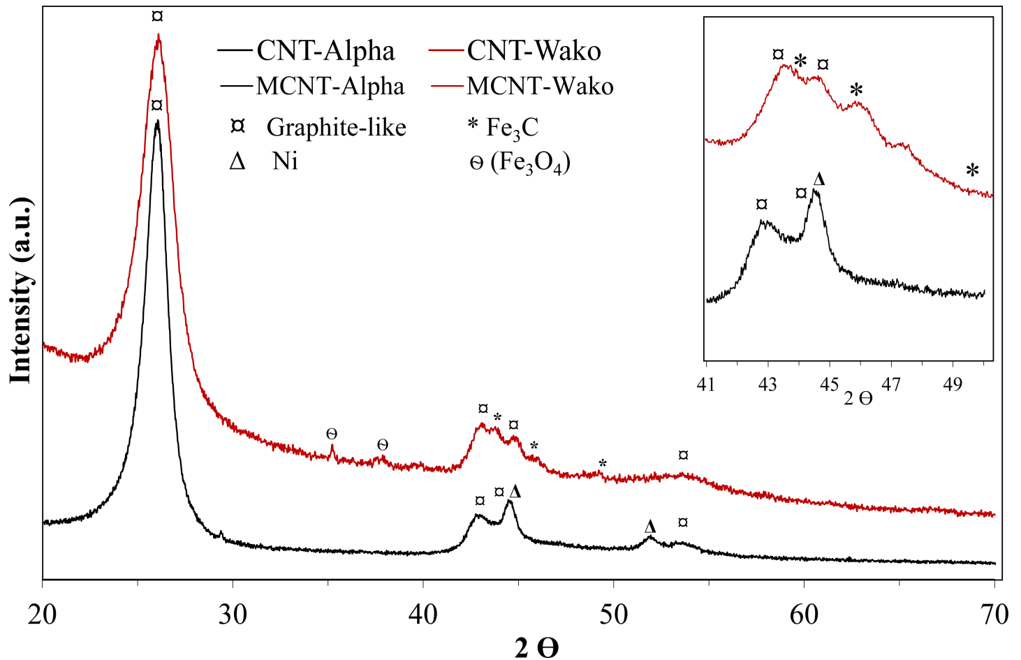
Fig 6. XRD traces of MCNT-Wako and MCNT-Alpha. The inset is enlargement of the range with most intense Fe/Ni diffraction peaks with a comparison among CNT-Wako, CNT-Alpha, MCNT-Wako and MCNT-Alpha.
