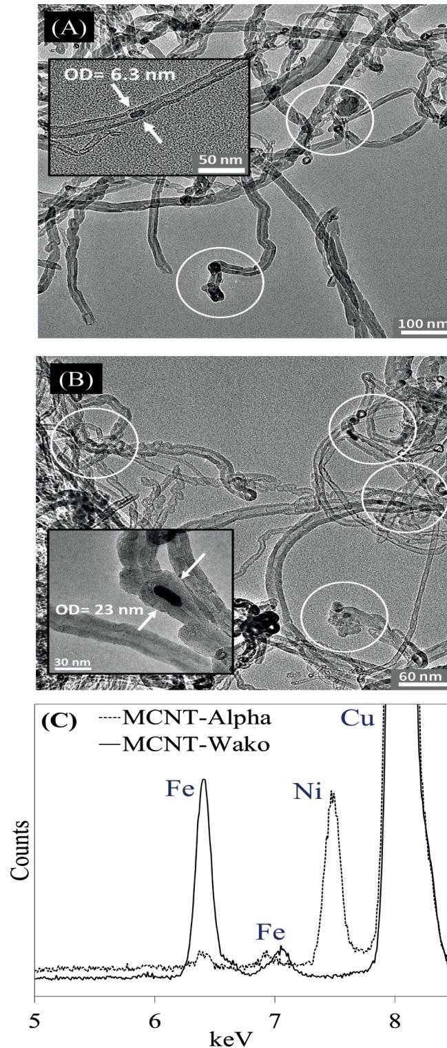
Fig 2. Low magnification micrographs of [A] MCNT-Wako and [B] MCNT-Alpha showing aggregates of CNT. The insets and white circles highlight the high-contrast particles containing metals within the CNT, and [C] EDX spectra for MCNT-Wako and MCNT-Alpha.
