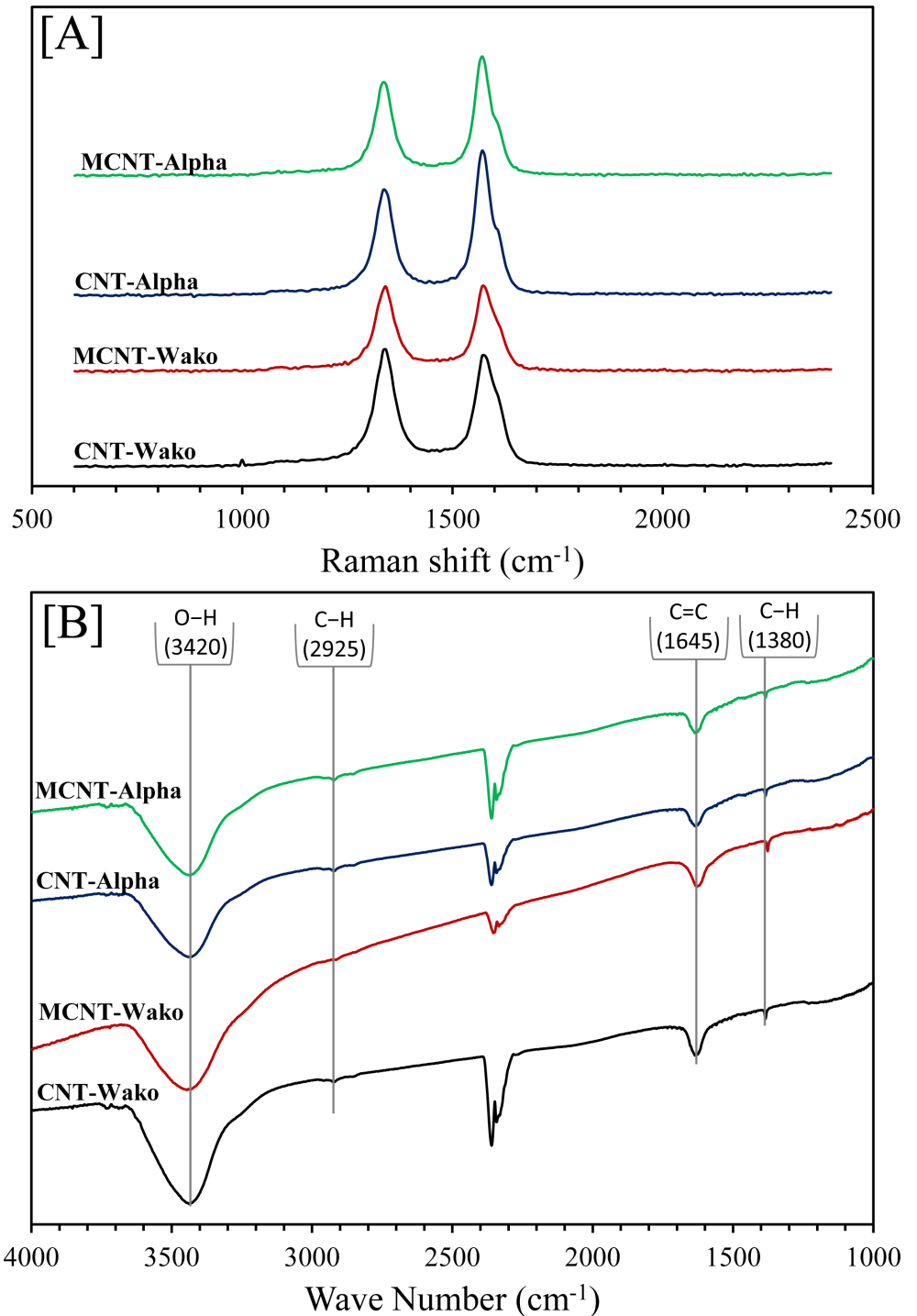
Fig 7. [A] The Raman spectra and [B] The FTIR spectra for CNT-Wako, MCNT-Wako, CNT-Alpha and MCNT-Alpha.
