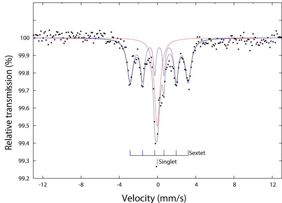
Fig 3. Mössbauer spectrum of MCNT-Wako at 293 K. The measurements are shown as black circles and the sum of the fitting components is shown as a black solid line. The peak positions (bar diagram) of the two fitting components (solid line in colours) are also shown.
