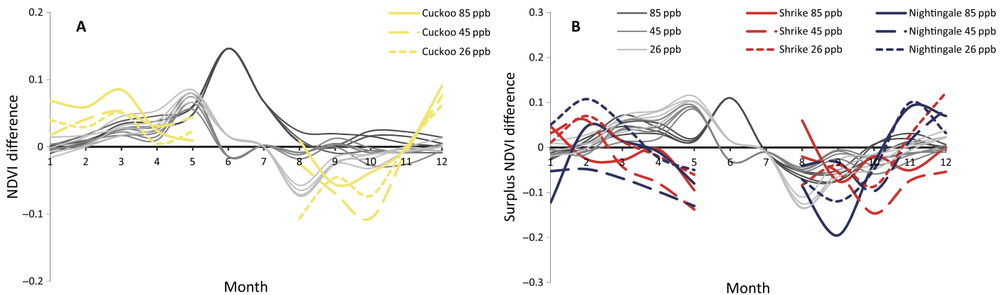
Fig. 4. Potential effects of future climate change on matching of resources along migratory tracks. Difference in projected (A) vegetation greenness, NDVI, and (B) vegetation surplus greenness, peak NDVI, along migratory tracks per month [1 (January) to 12 (December)] for 2011 and 2080 based on three climate change scenarios [26, 45, and 85 parts per billion (ppb) atmospheric CO 2 ]. We used biweekly projected data on precipitation and temperature to model NDVI. Simulated tracks traversed 100° to 160° of latitudes in total (starting at 55°N, 9°E), corresponding to a trans-Saharan migration (indicated by the four gray lines). The differences between the projected vegetation greenness for tracks in 2011 and 2080 of common cuckoos (yellow lines) and projected surplus vegetation greenness for shrikes (red lines) and nightingales (blue lines) are shown for comparison with the simulated random tracks. Positive values indicate expected improvement of environmental conditions (NDVI and peak NDVI) by 2080, and negative values indicate impoverished conditions or a mismatch. Breeding season data are omitted because of aberrant projections due to a low proportion of land cover.
