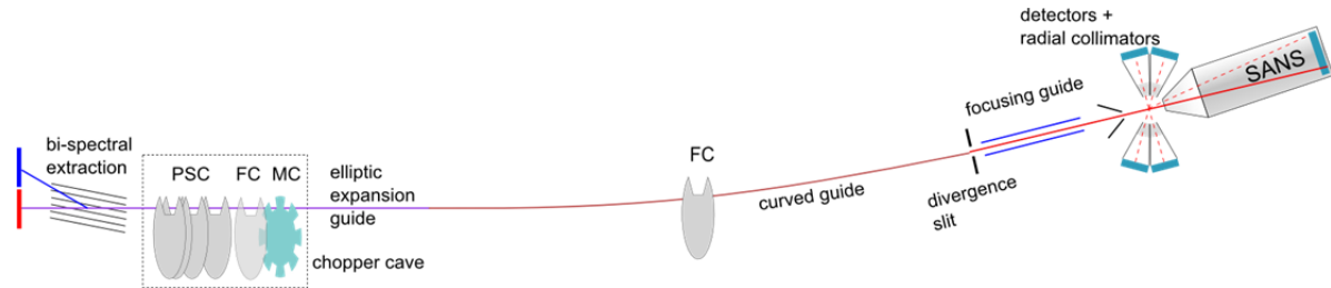
Figure 1: Schematic drawing of the BEER layout with the key components, e.g. pulse shaping (PSC), frame definition (FC) and modulation choppers (MC): for details see the text.
