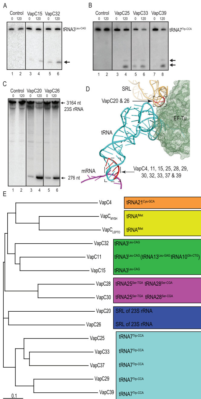
Figure 7. Phylogeny can predict cellular VapC targets. (A) Detection of in vivo cleavage of tRNA3 Leu-CAG by VapC15 and VapC32 by Northern analysis was performed as in Figure 3 (D); VapC expression was induced from M. smegmatis MC 2 155 carrying plasmids pMEND::vapC15::HTF or pMEND::vapC32::HTF. (B) in vivo cleavage of tRNA Trp-CCA by VapC25, VapC33 and VapC39 was detected by Northern analysis performed as in Figure 5 (B). Toxin expression was induced from plasmid pMEND::vapC25::HTF, pMEND::vapC33::HTF and pMEND::vapC39::HTF. (C) Cleavage of 23S rRNA detected by Northern analysis was performed on RNA purified from M. smegmatis strain MC 2 155 containing plasmids pMEND::vapC20::HTF and pMEND::vapC26::HTF. Cell samples were collected before (indicated by 0) and after 120min of induction (indicated by 120) and analysed as described in Materials and Methods. The arrow indicates the 276 nucleotide cleavage product of 23S rRNA generated by VapC20 and VapC26, as mapped previously (22). The full-length 23S rRNA (3164 nt) is also indicated with an arrow. (D) Region of the decoding center of 70S ribosome
