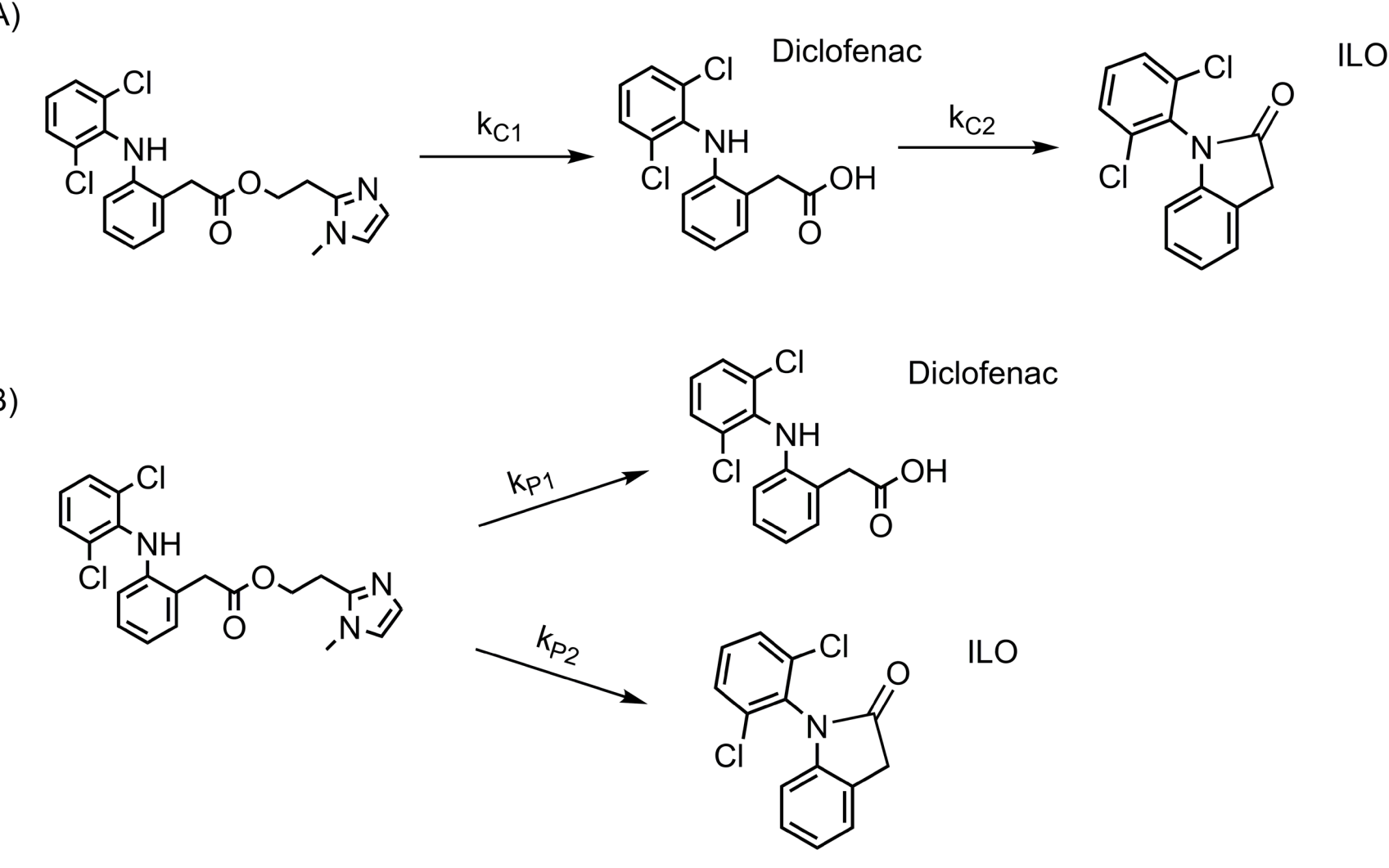
Figure 4: Reaction schemes for formation of diclofenac and ILO from degradation of the DP-2 prodrug at pH below 2 (A) and at 5.8 \leq \text{pH} \leq 10 (B) and 37°C.
