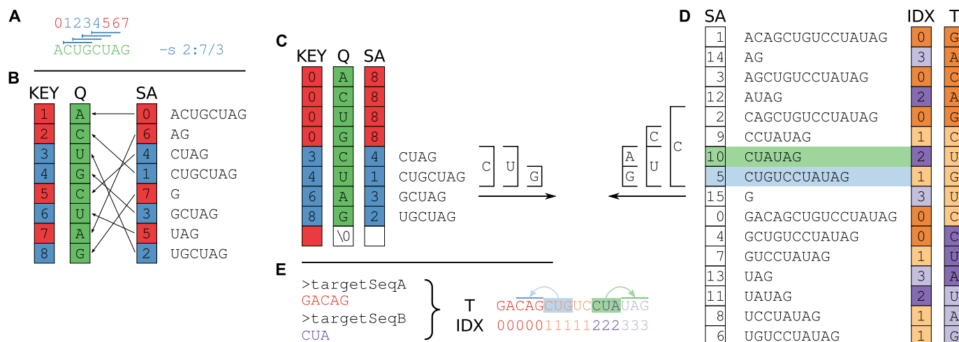
Figure 2. Suffix array preparation and matching. (A) The user provides a query ( Q = ACUGCUAG of length m = 8 ) and specifies the seed by either length, position, or both. The command-line parameter -s 2:7/3 requires a seed to be at least 3 nt long and located between positions 2–7 of the query. This allows for only four valid seed start locations, indicated with the blue lines above the query sequence. This corresponds to positions 1–4 in the 0-based index being valid start positions that satisfy the seed requirements, colored blue. Seeds starting in any other position would violate the seed requirements and are colored red. (B) A suffix array of the query ( SA ) is constructed, containing the starting positions of suffixes of Q in lexicographical order. KEY holds a running number; boxes are colored blue if the suffixes satisfy the seed requirements, red otherwise. Q is stored as the original sequence, regardless of the SA order. (C) Suffixes that violate the seed requirement (see A) are set to zero in KEY and m in SA , pointing to the null terminator. The array is then re-sorted based on KEY . This ensures that all discarded suffixes are moved to the beginning of the array, while all valid suffixes are still sorted in lexicographical order. (D) The target SA is built from the concatenated sequences, as shown in Supplementary Figure 1. IDX is sorted according to SA order, while T is stored in order of the original sequence. For both query and target SA , we find the intervals of suffixes starting with each nucleotide. In the example, we show the suffixes starting with C and further traverse both SA s as long as there are corresponding non-empty intervals (between (C) and (D)), until the minimum seed length is reached. We find two positions in the target that match the CUG in the query, highlighted in light green and blue respectively. Note that the query suffix CUAG would also match the target CUA , but not CUG . (E) The match with IDX 2 (light green) refers to a target site in the reverse complement sequence 3, and likewise IDX 1 to a target site in 0 (light blue).
