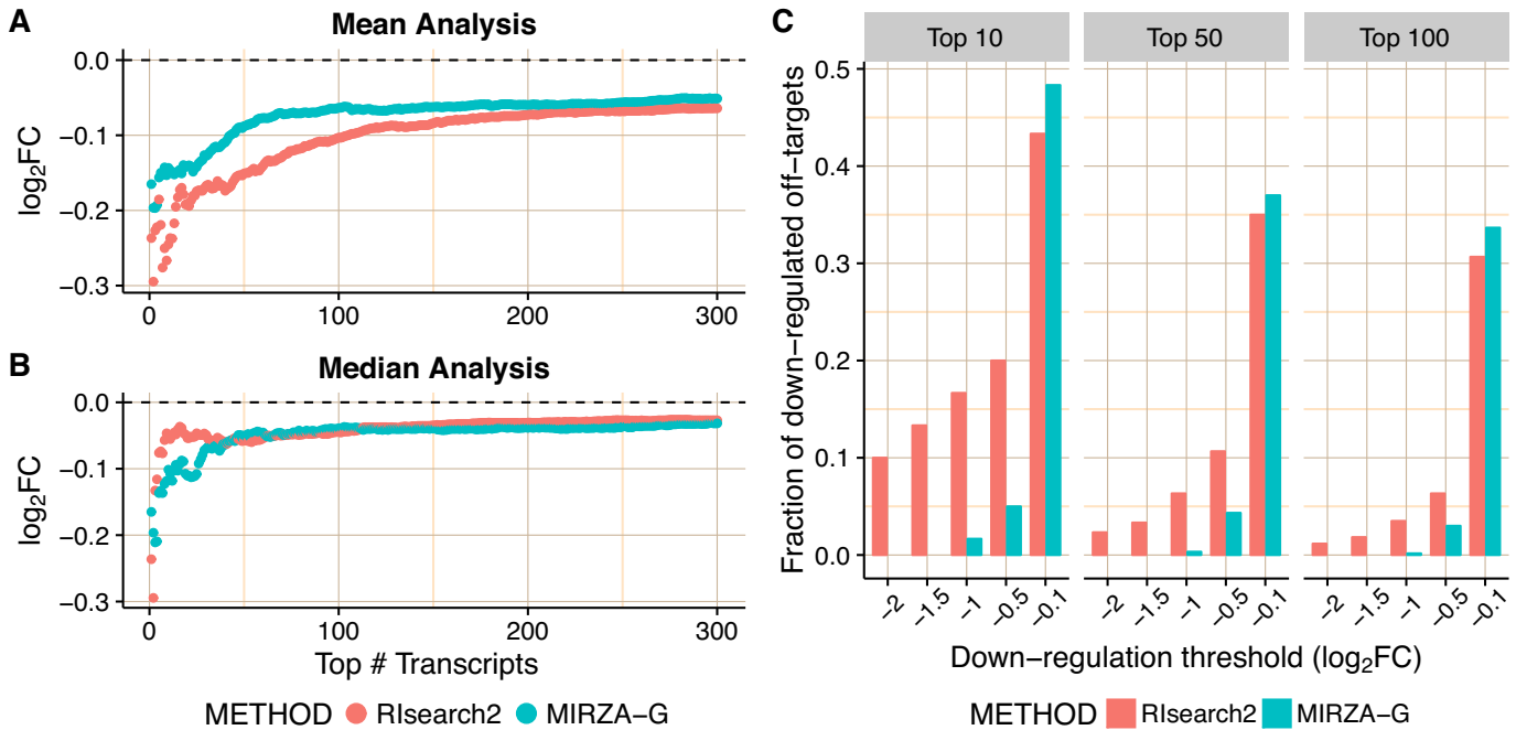
Figure 3. Evaluation of individual off-target predictions performed by RIsearch2 (siRNA off-targets pipeline) and MIRZA-G. All analyses are based on the Burchard dataset where six APOB siRNAs were transfected into PLC/PRF/5 cell lines. Top off-targets are selected from method-specific predictions based on the confidence scores generated by either method ( p_{off,j} for RIsearch2). In the mean (A) and the median (B) fold changes analyses, mean/median differential expression level (averaged over all siRNAs) of top off-targets are plotted for different numbers of top off-targets considered. (C) Proportion of critical off-targets within the top (10, 50, 100) predictions generated by either method for six siRNAs, i.e. considering 60 transcripts in total for top 10. Off-targets are considered critical if they are downregulated, upon the transfection of siRNA, with a \log_2FC value lower than the threshold given in the x-axis.
